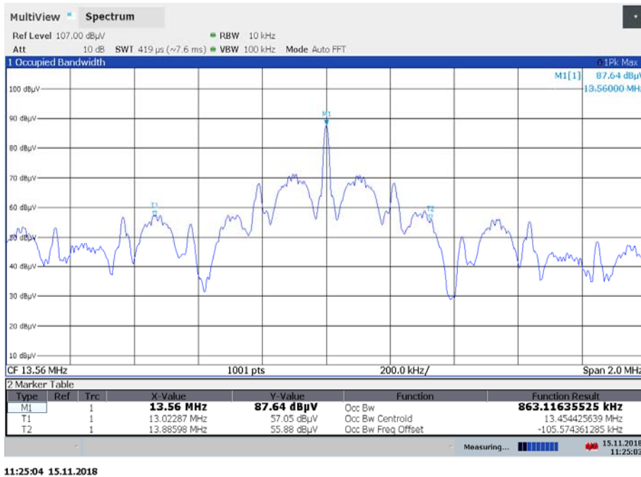
Plot 2: 99 % emission bandwidth, EUT with tag type 1
