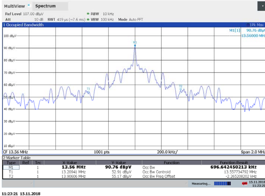
Plot 1: 99 % emission bandwidth, EUT without tag
