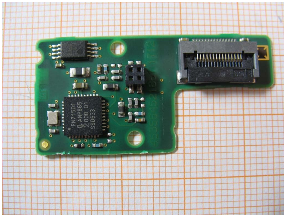
Photo 6: EUT
