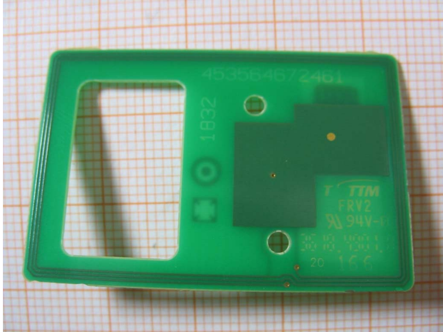
Photo 5: EUT
