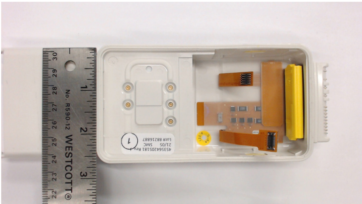
Inside View of MX40 Rear Case, FCC ID: PQC-MX40SH2C4
