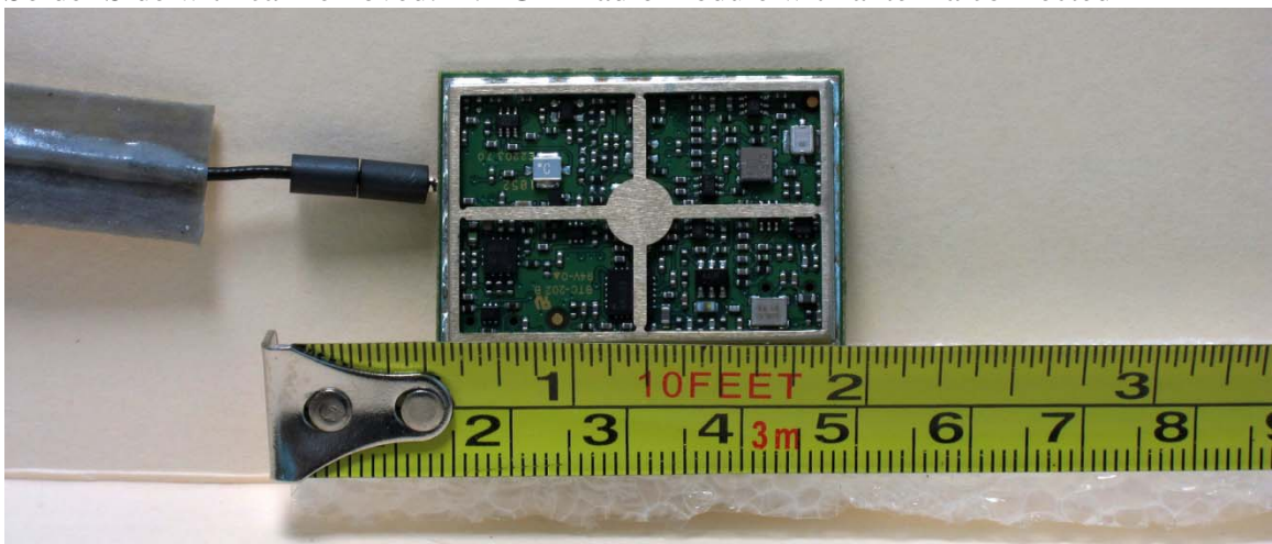
Solder Side with can removed: 1.4 GHz radio module with antenna connected
