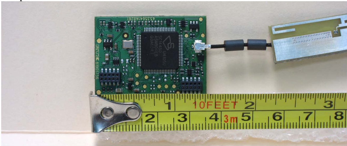
Component side with antenna connected
