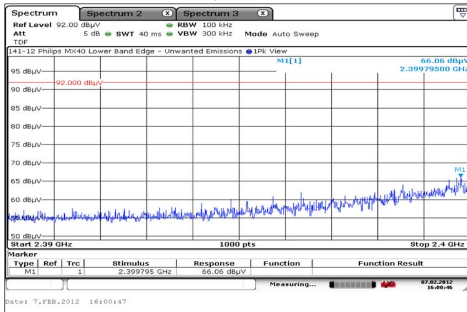
Measurement Plot – Lower Band Edge – Unwanted Emissions
