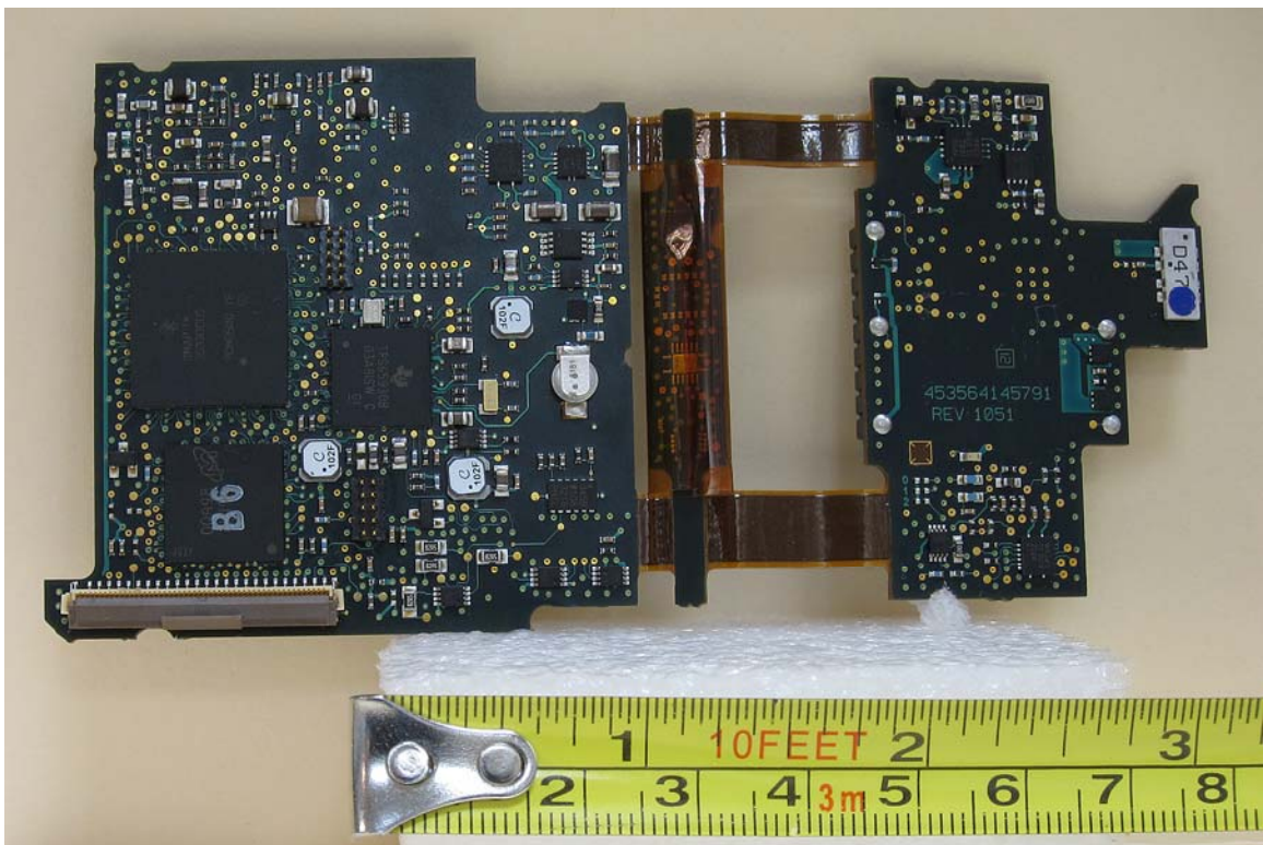
Main board
