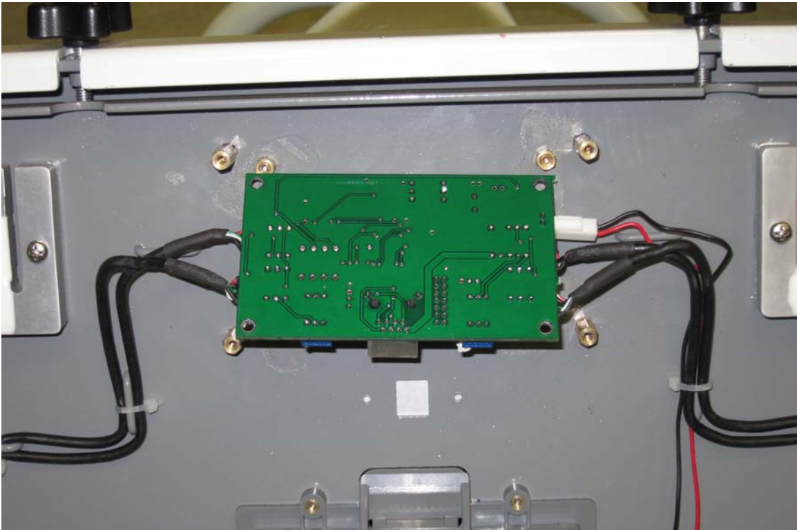
Wetboard Rear
