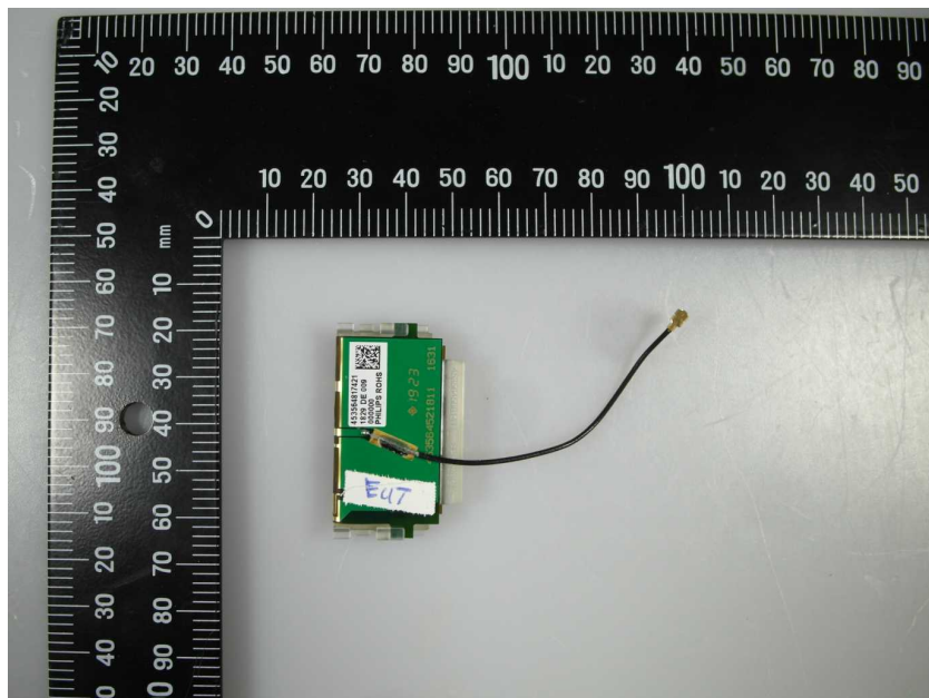
Photo 12: Antenna Apollo
