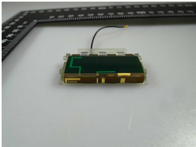
Photo 14: Antenna Apollo
