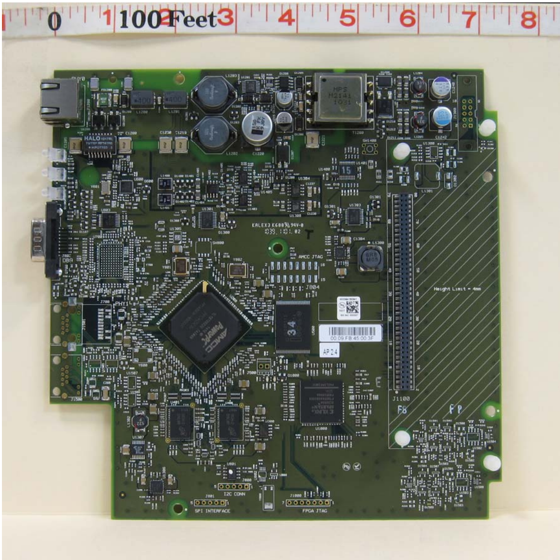
Main Board Front
