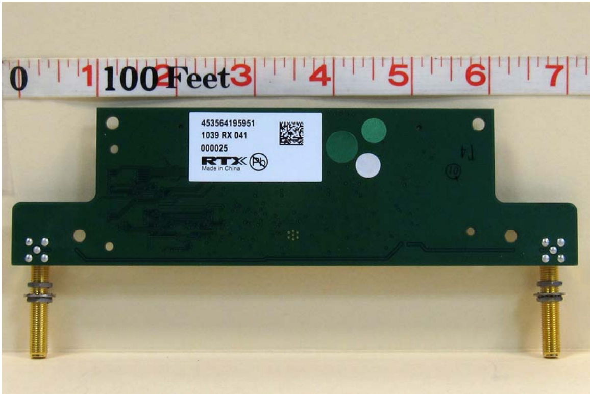
Transmitter Board – Rear
