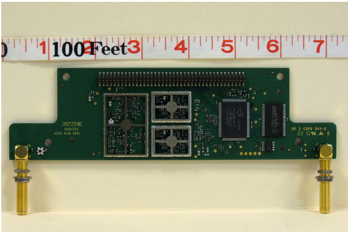
Transmitter Board – Front covers Off
