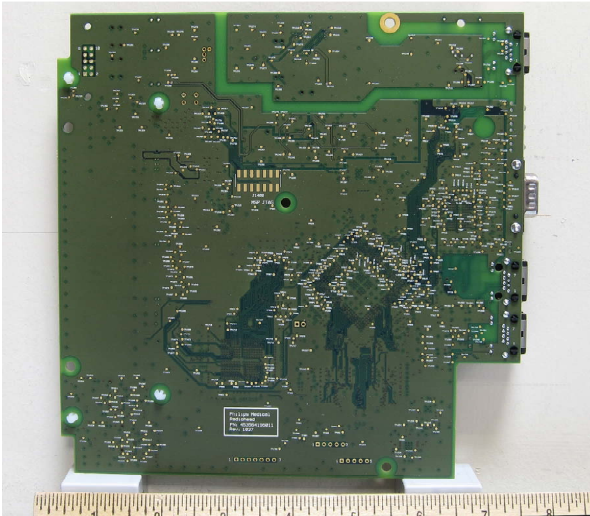
Mainboard Rear
