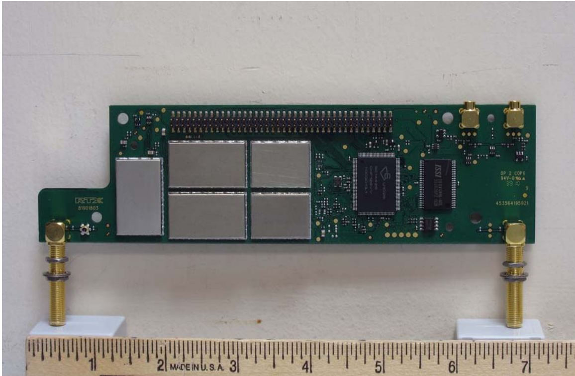
Transmitter Board Rear
