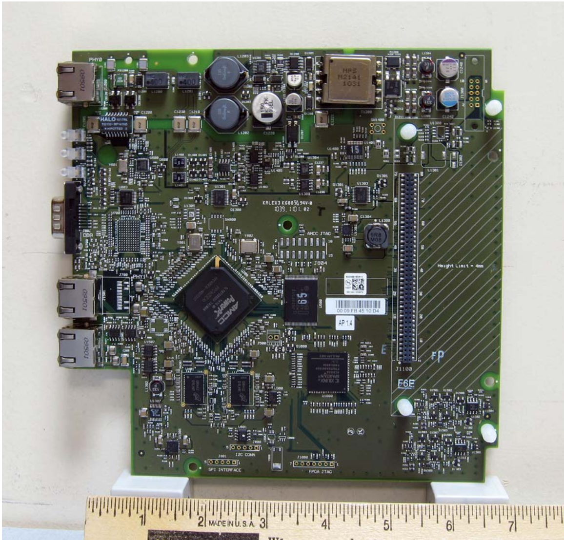
Mainboard Front
