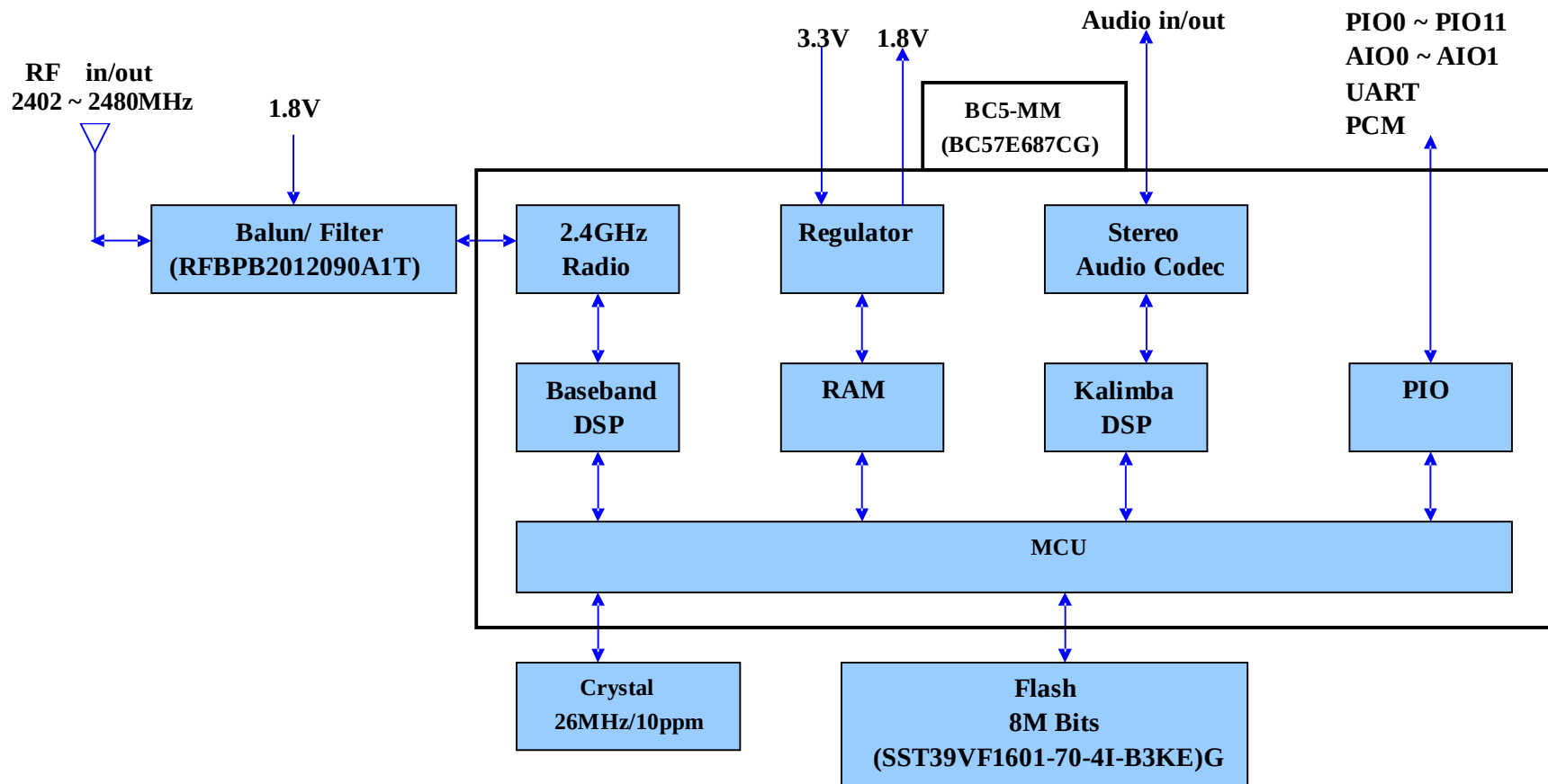
BTM512 Block Diagram
