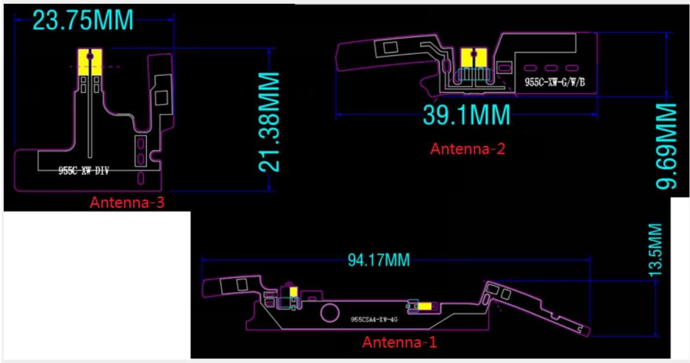
1-1. Antenna size diagram
