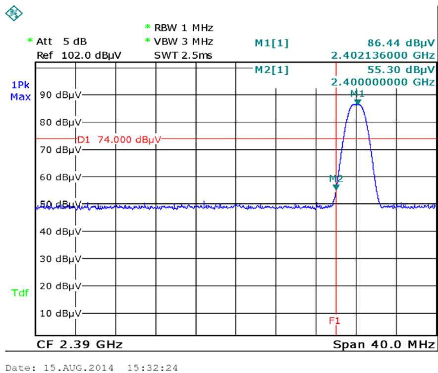
Left Side-PK
