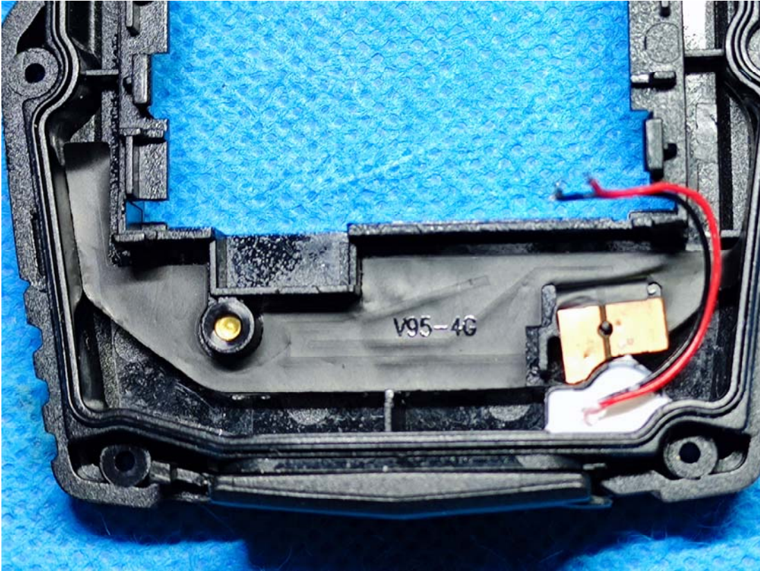
2G/3G Antenna
