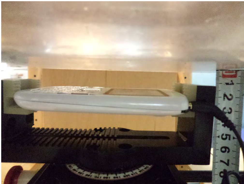
Body-worn-Headset Front Setup Photo (15mm)
