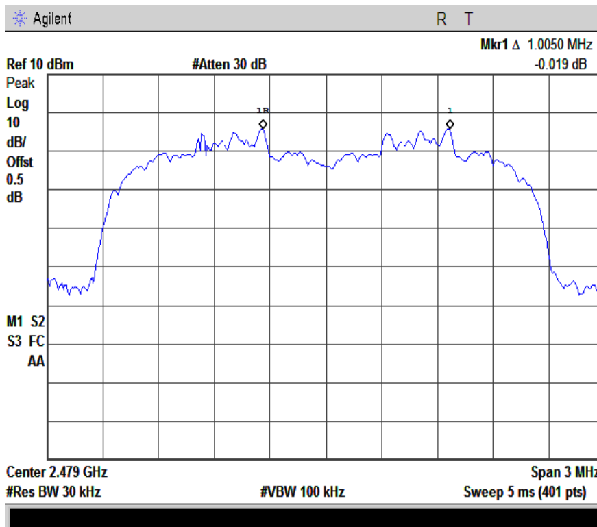
3M-Channel Separation-2480
