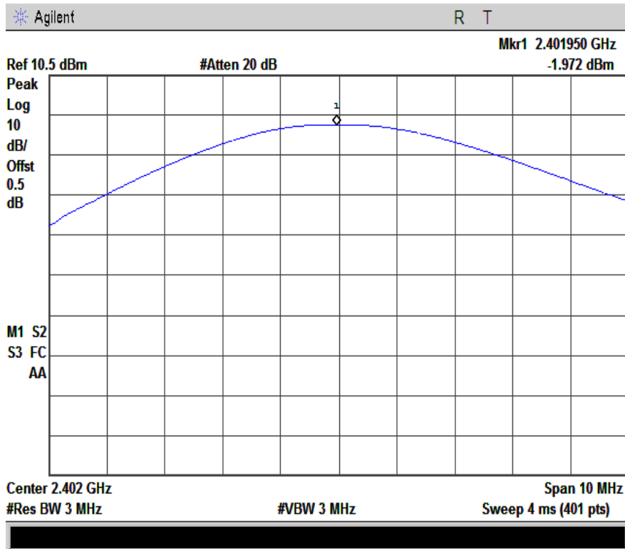
1M-power-2402
