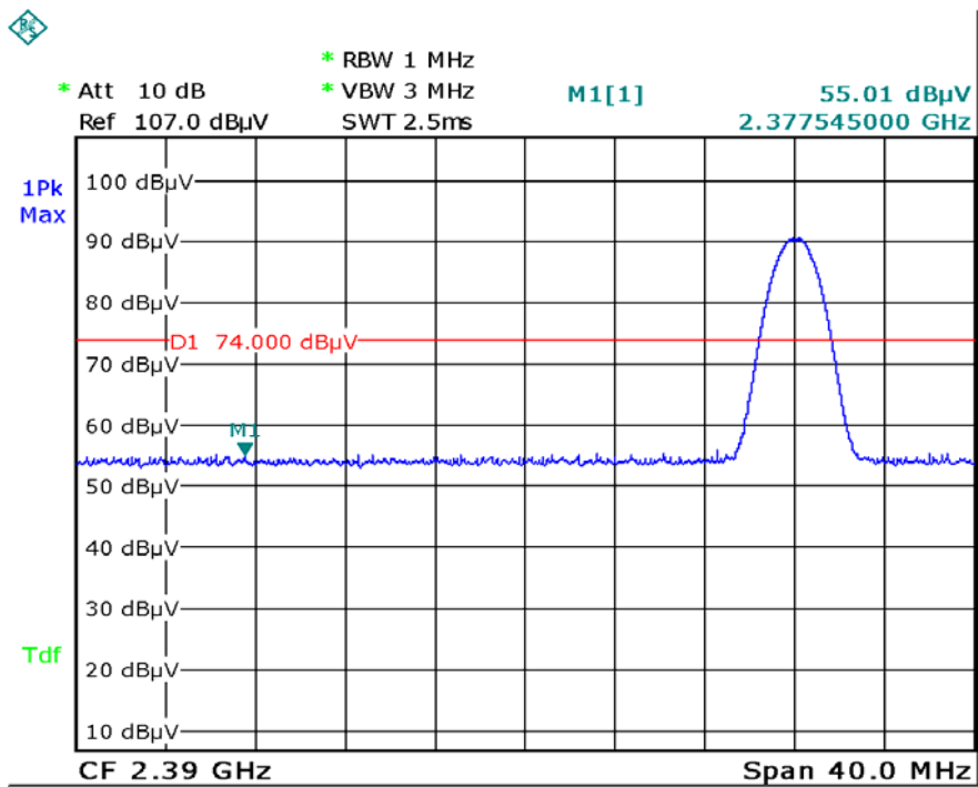
2M-L-PK
