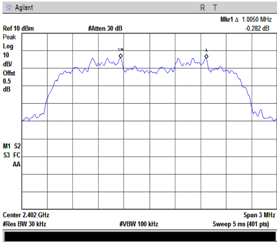
2M-Channel Separation-2402
