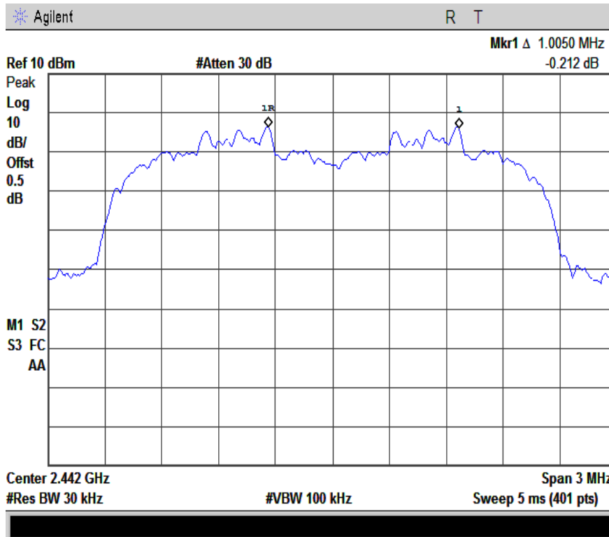
3M-Channel Separation-2441
