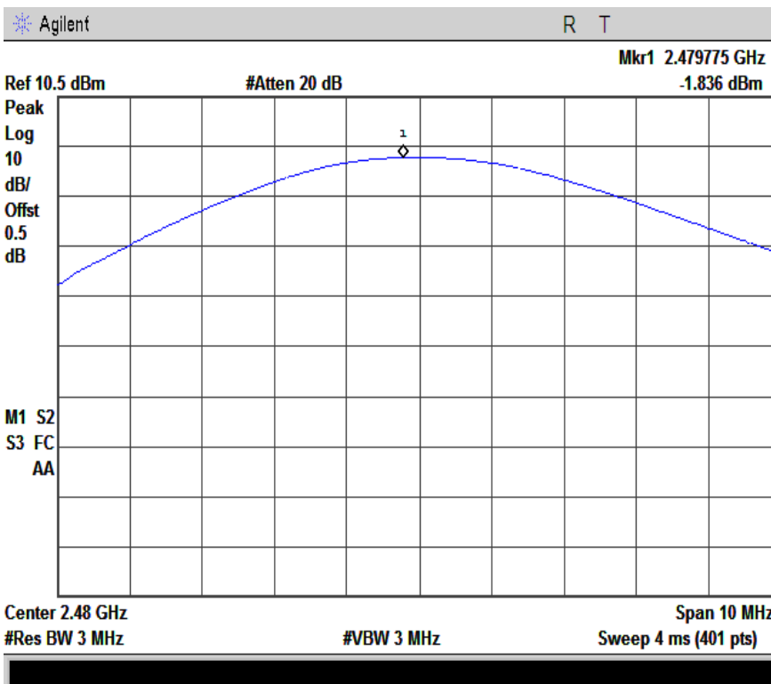
1M-power-2480
