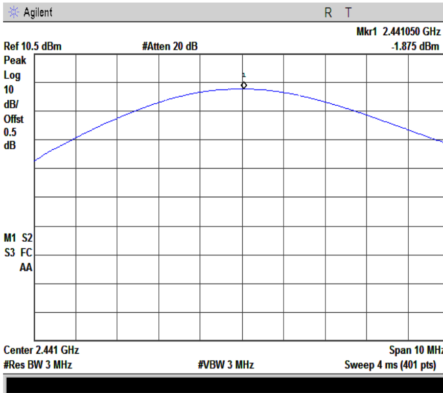
2M-power-2441
