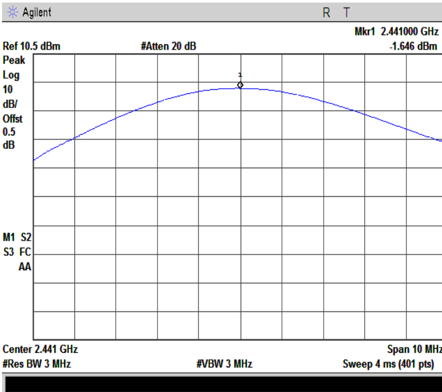
3M-power-2441
