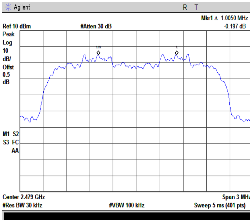
2M-Channel Separation-2480
