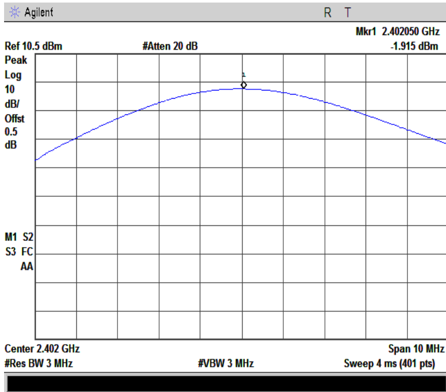
3M-power-2402
