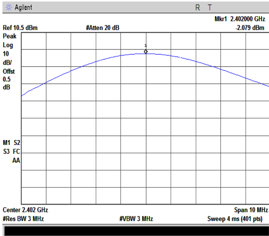
2M-power-2402
