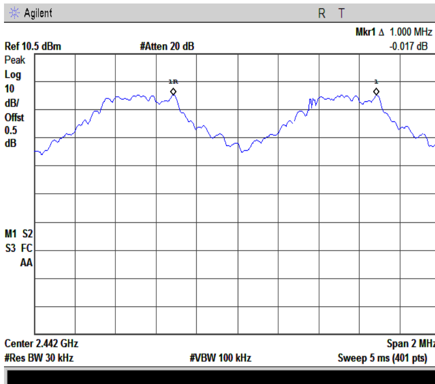
1M-Channel Separation-2441
