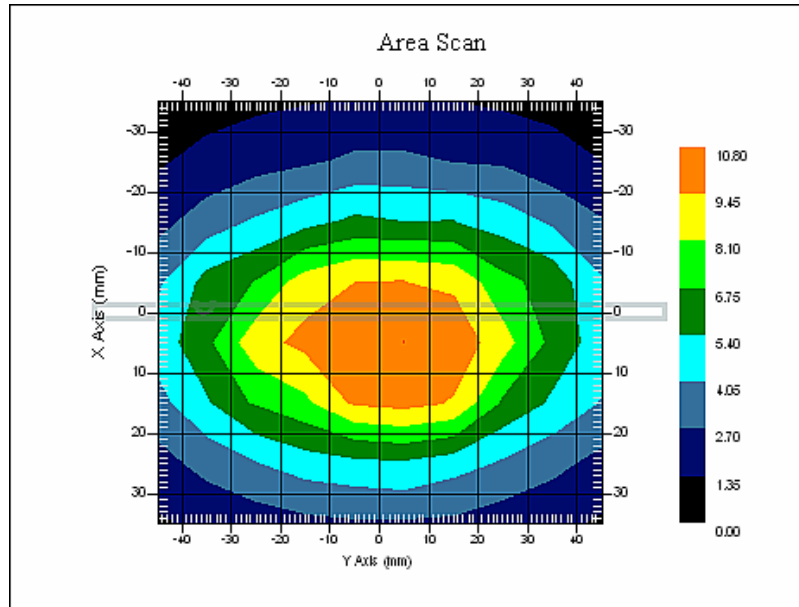
835 MHz System Validation with Body Tissue
