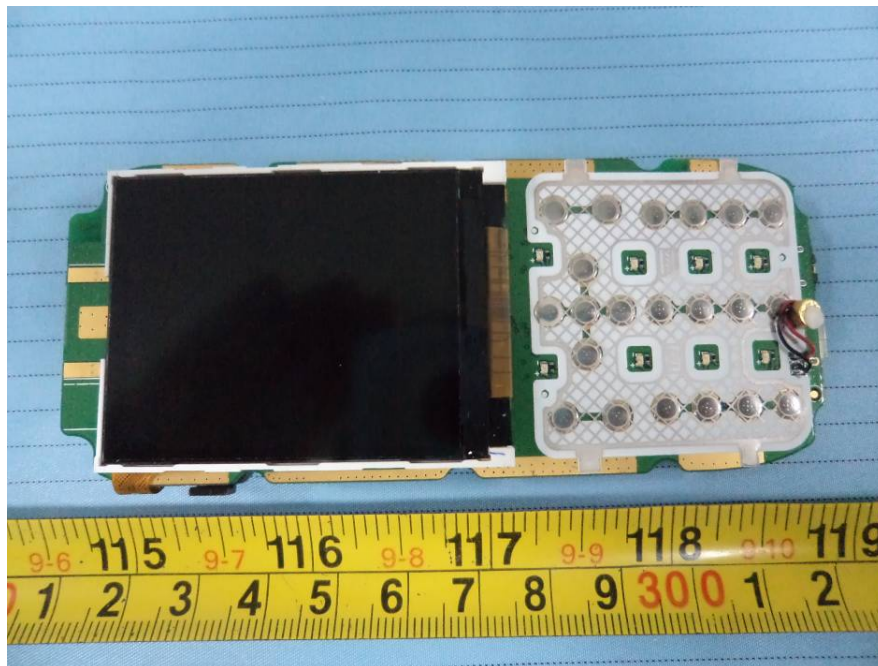
EUT – Main Board Top with LCD and Keyboard View
