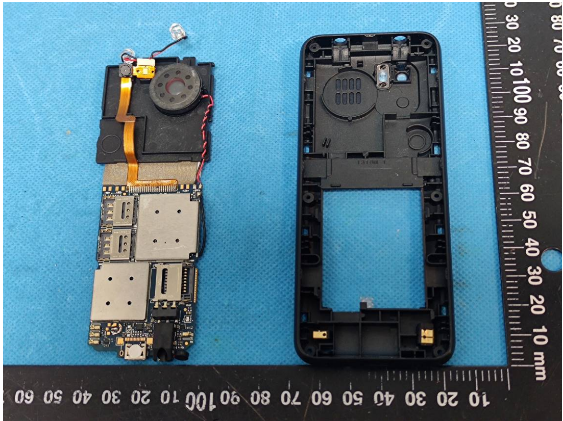
Main Antenna
