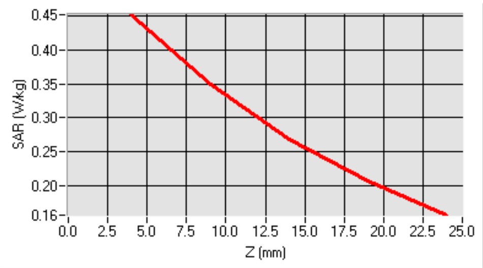
SAR, Z Axis Scan (X = -1, Y = -49)
