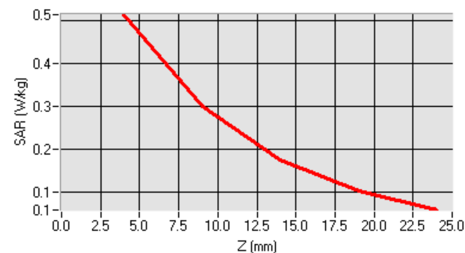
SAR, Z Axis Scan (X = -14, Y = -57)
