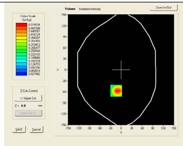
SAR, Z Axis Scan (X = -14, Y = -57)
