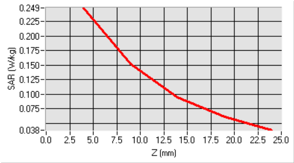
SAR, Z Axis Scan (X = -56, Y = -54)
