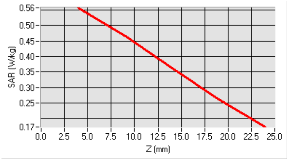
SAR, Z Axis Scan (X = -55, Y = -32)
