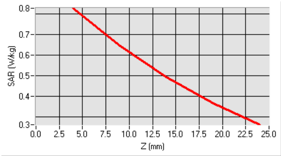
SAR, Z Axis Scan (X = -5, Y = -47)
