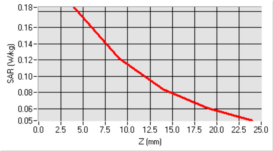
SAR, Z Axis Scan (X = -56, Y = -16)
