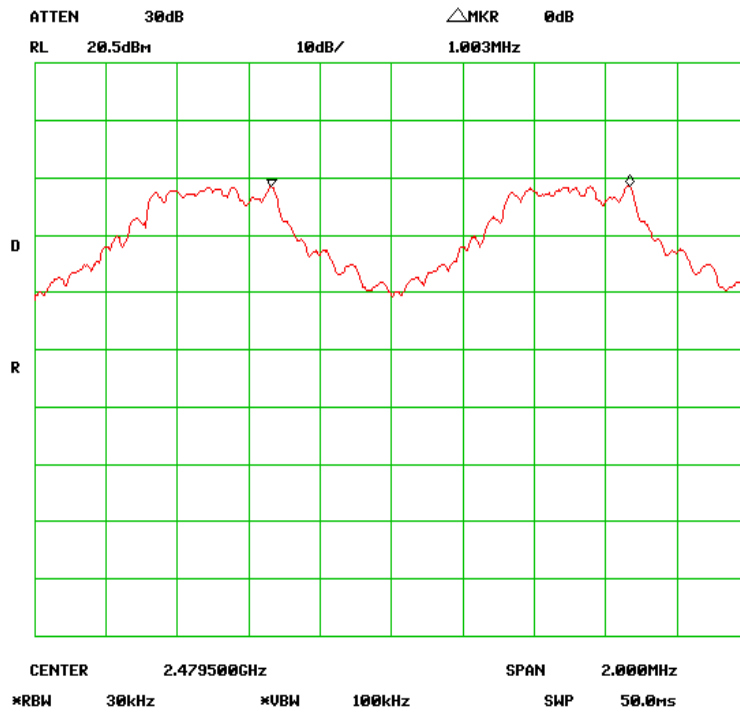
1M-Channel Separation-2480
