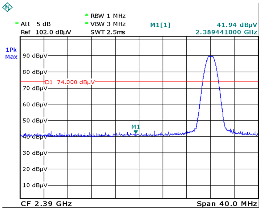
1M-Left Side-PK
