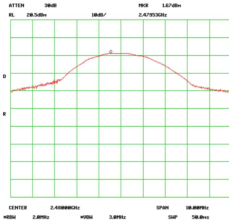
1M-power-2480
