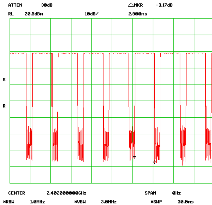
DH5-2402
