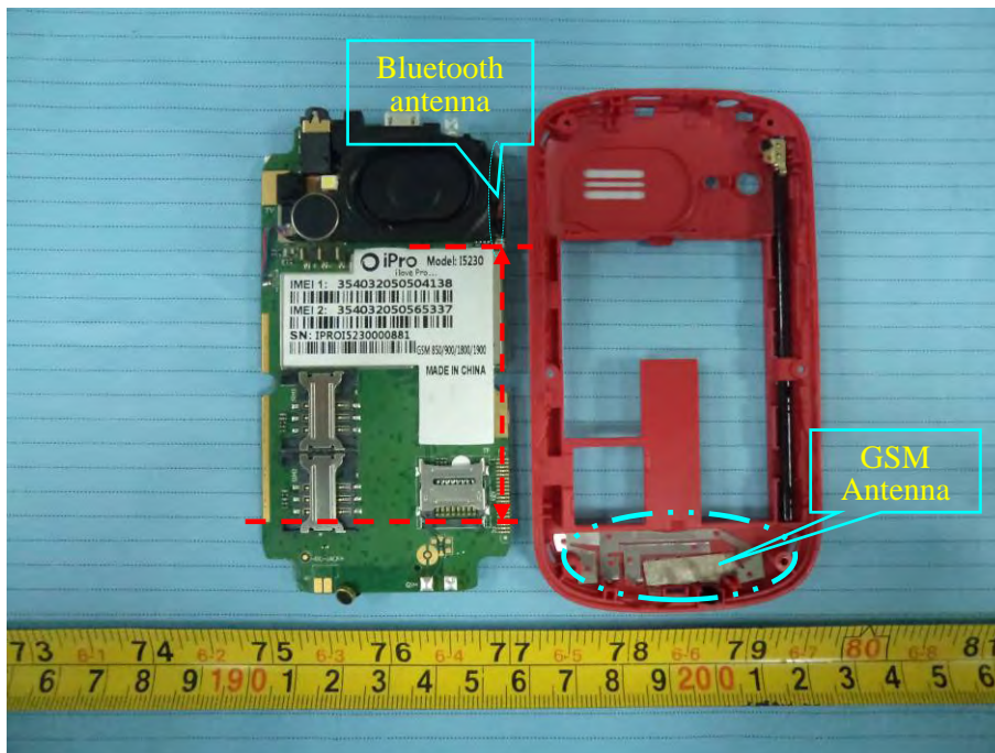
Bluetooth and GSM Antenna Location
