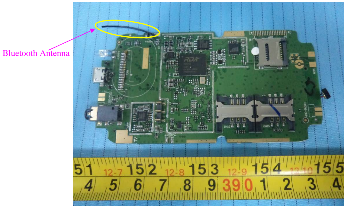
EUT – Main Board Bottom Shielding off View
