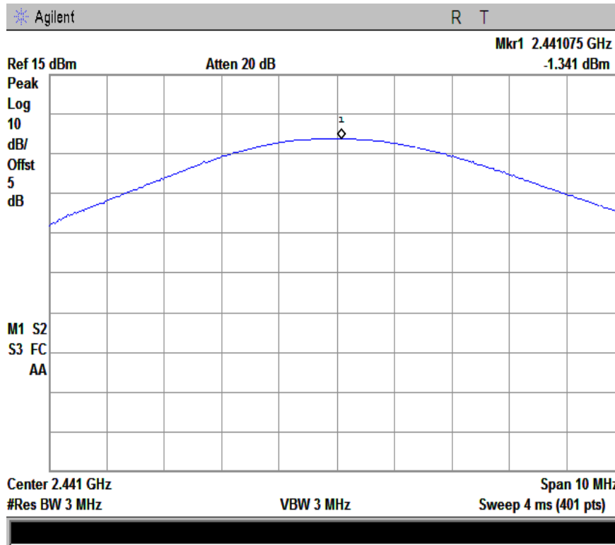
1M-power-2441
