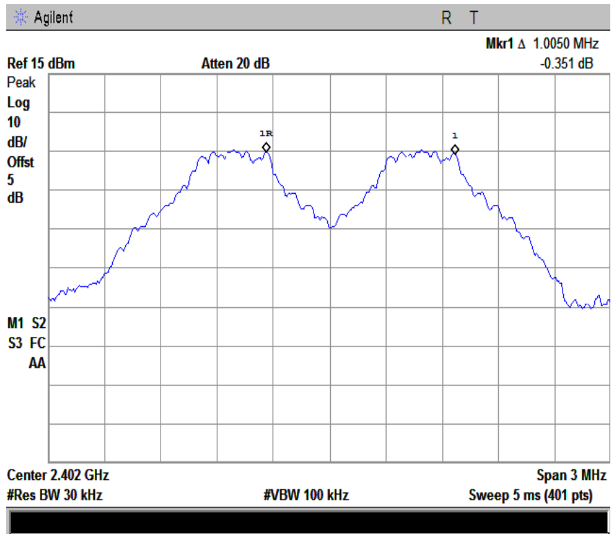
1M-Channel Separation-2402
