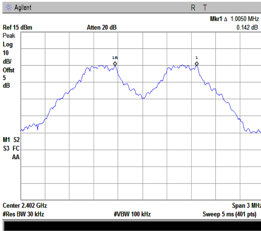
1M-Channel Separation-2402
