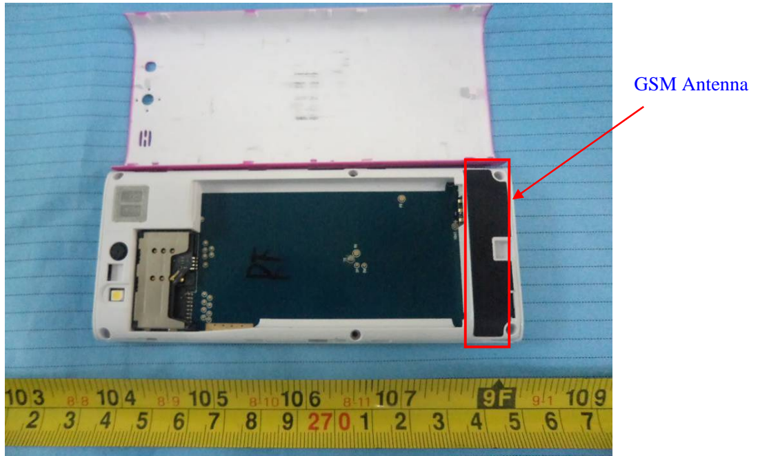
EUT – Battery off View
