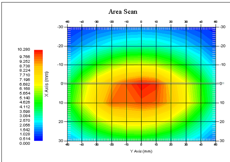
835 MHz System Validation with Body Tissue
