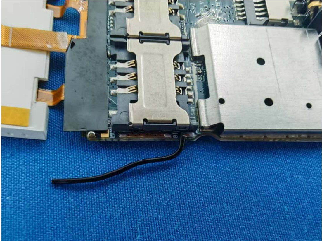
Bluetooth Antenna
