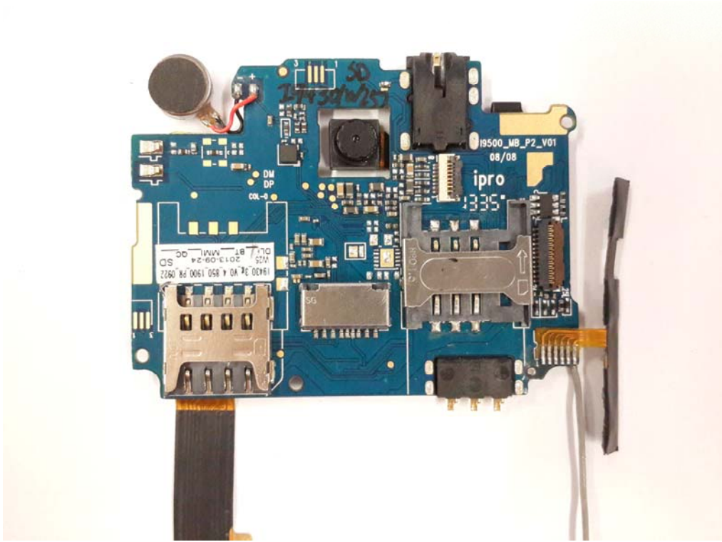
PCB Back
