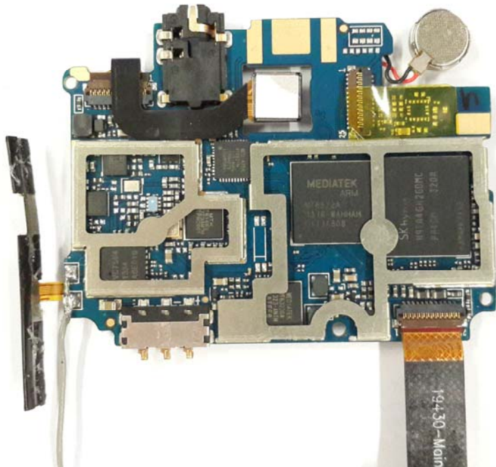
PCB Front
