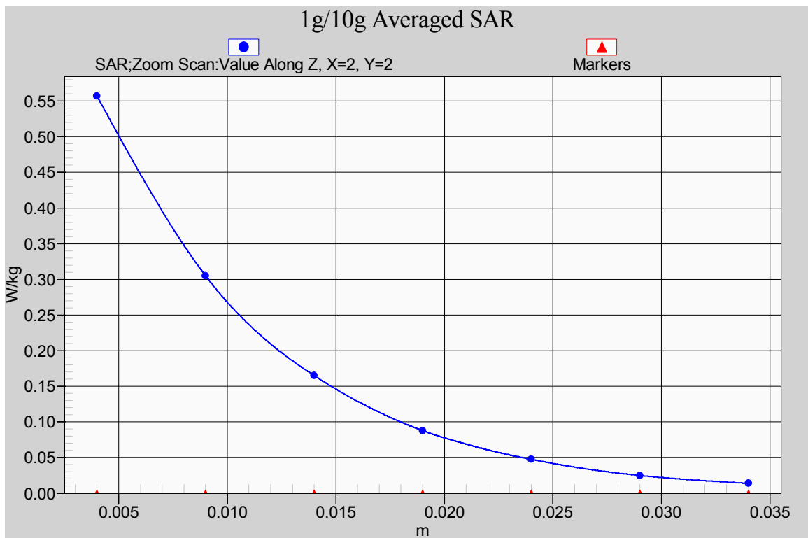
Fig. 57-1 Z-Scan at power reference point (2450 MHz CH11)
