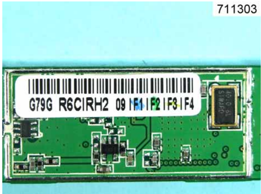
Wistron: PIFA Antenna (INTERNAL) / 3.00 dBi
