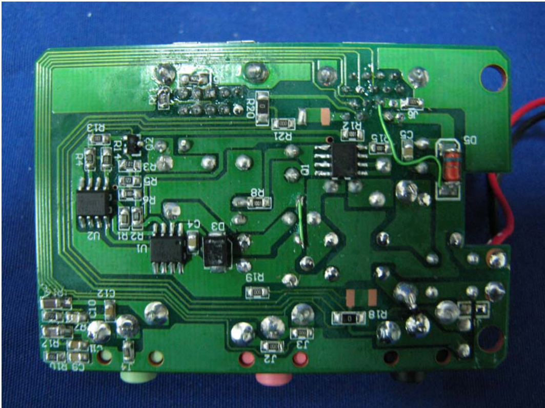
(55) EUT Photo
