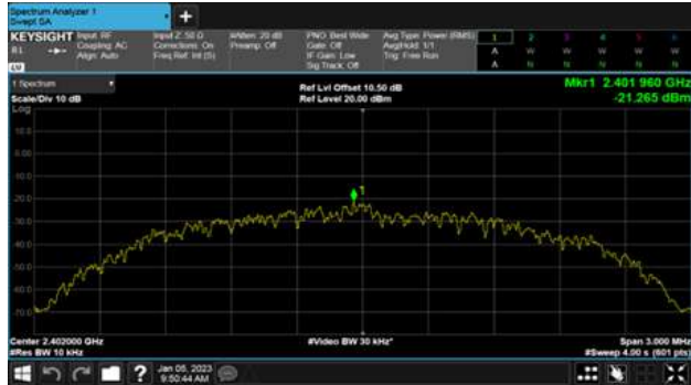
Modulation Type: GFSK(2Mbps) CH00
