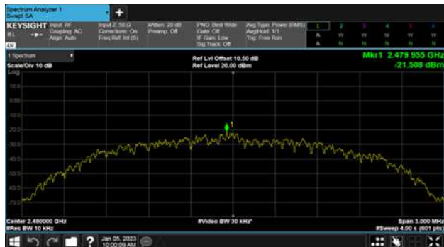
Modulation Type: GFSK(2Mbps) CH39
