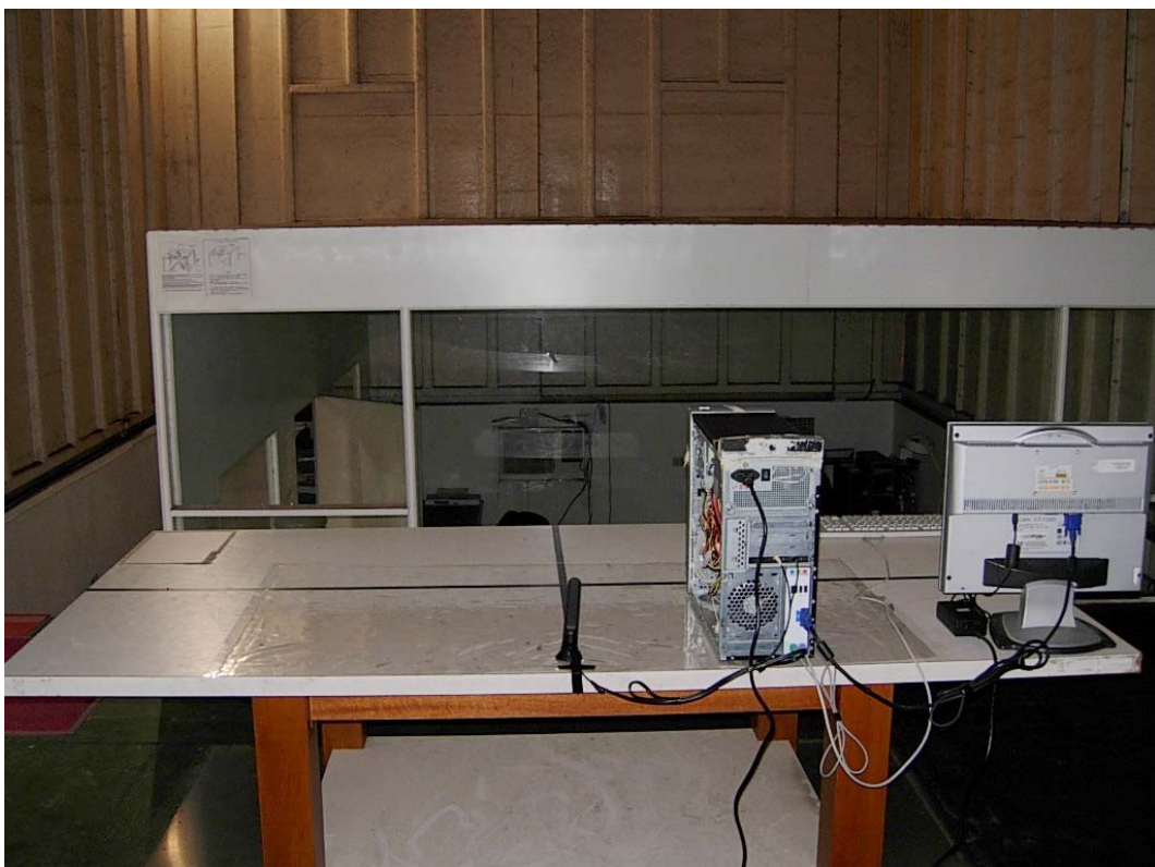
Back View of Radiated Test – Mode 1 ~ Mode 4
