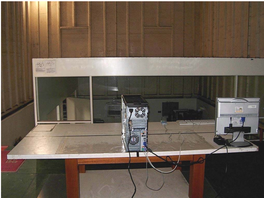
Back View of Radiated Test – Mode5 ~ Mode 8
