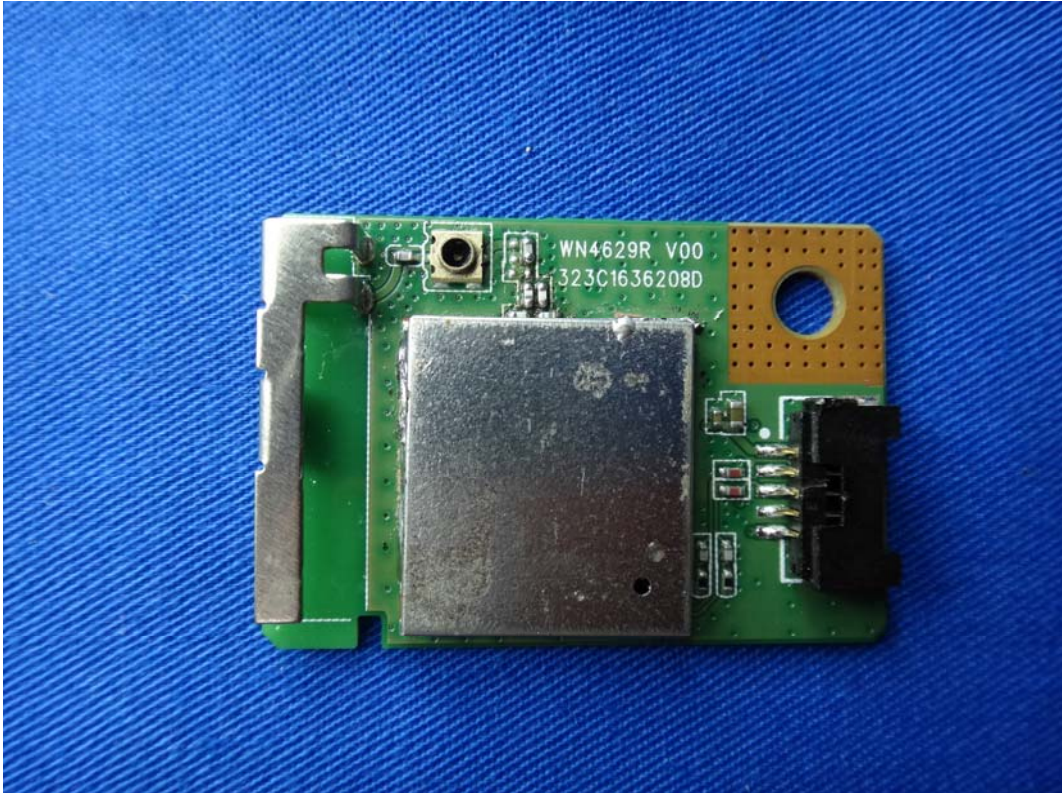
(1) EUT Photo
