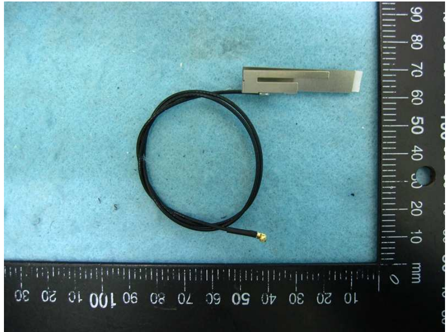
Ant. 2: 400mm
