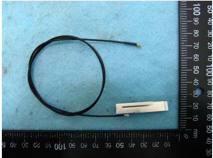
Ant. 6: 600mm
