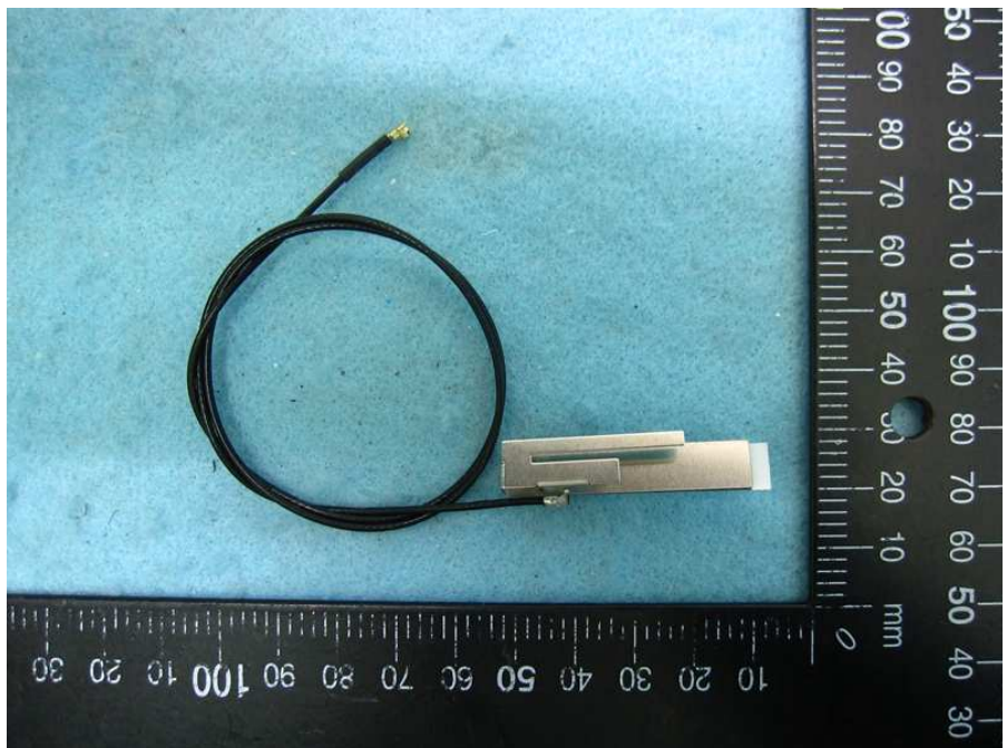
Ant. 3: 450mm
