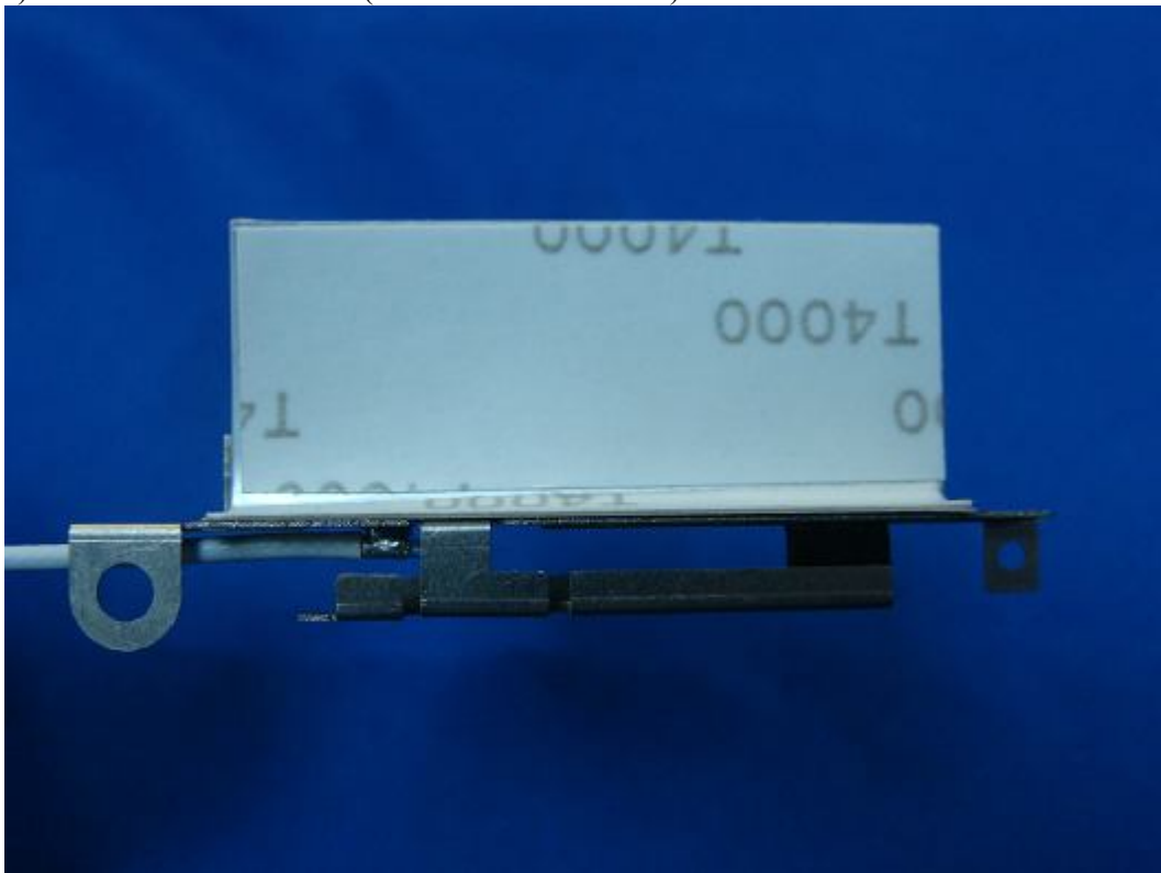
(12) EUT Photo –Antenna 1 (Without metal reflector)
