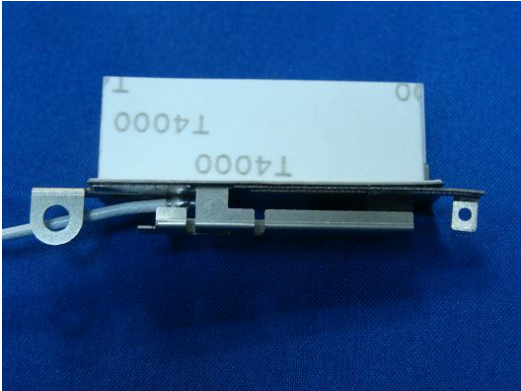
(16) EUT Photo –Antenna 1 (Without metal reflector)
