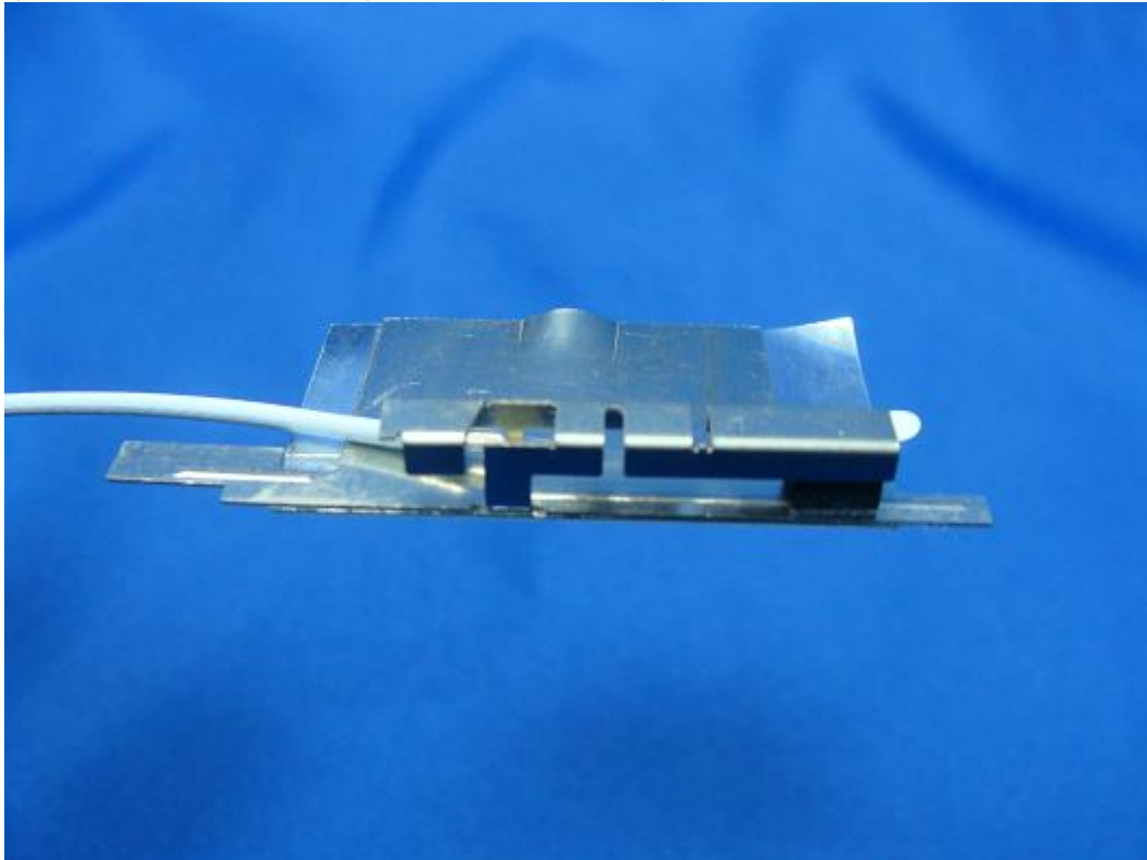
(21) EUT Photo –Antenna 2 (Without metal reflector)
