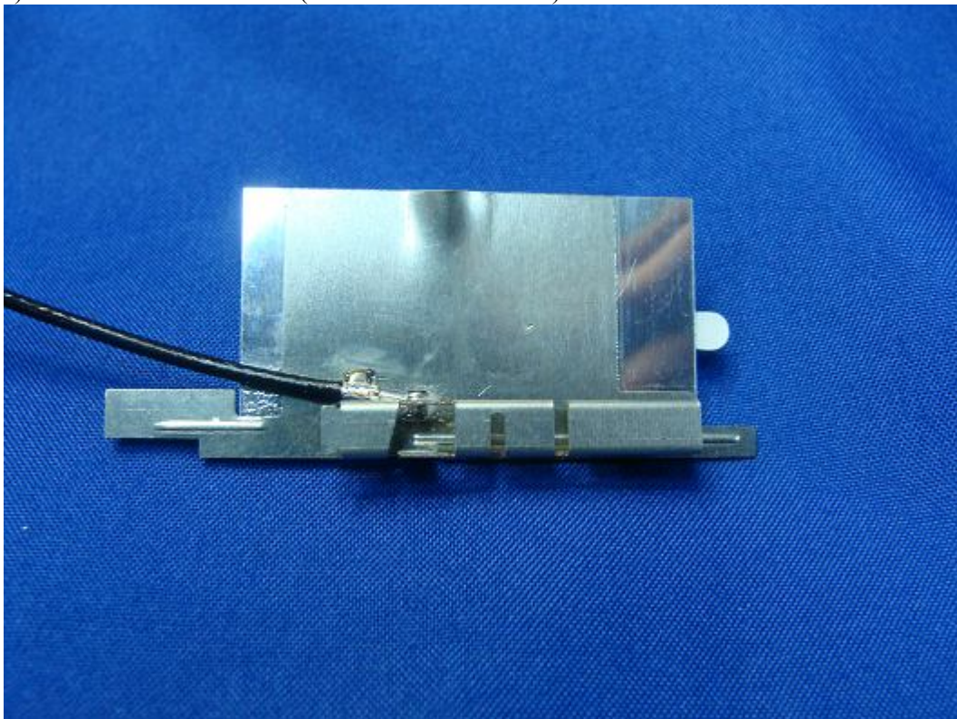
(22) EUT Photo –Antenna 2 (Without metal reflector)
