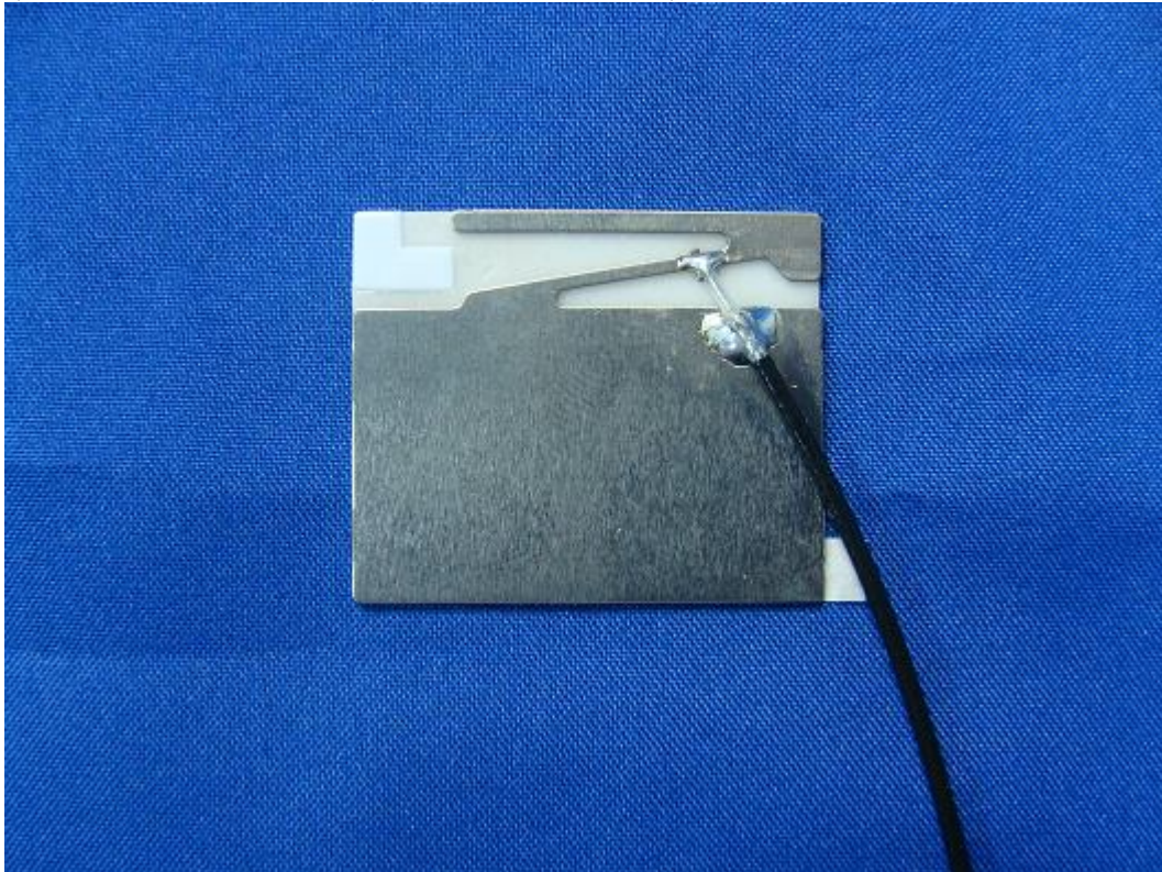
(30) EUT Photo –Antenna 3 (Without metal reflector)
