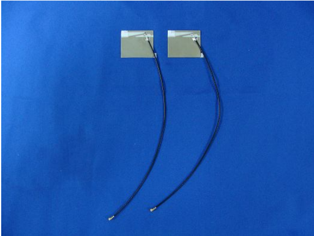
(26) EUT Photo –Antenna 3 (Without metal reflector)
