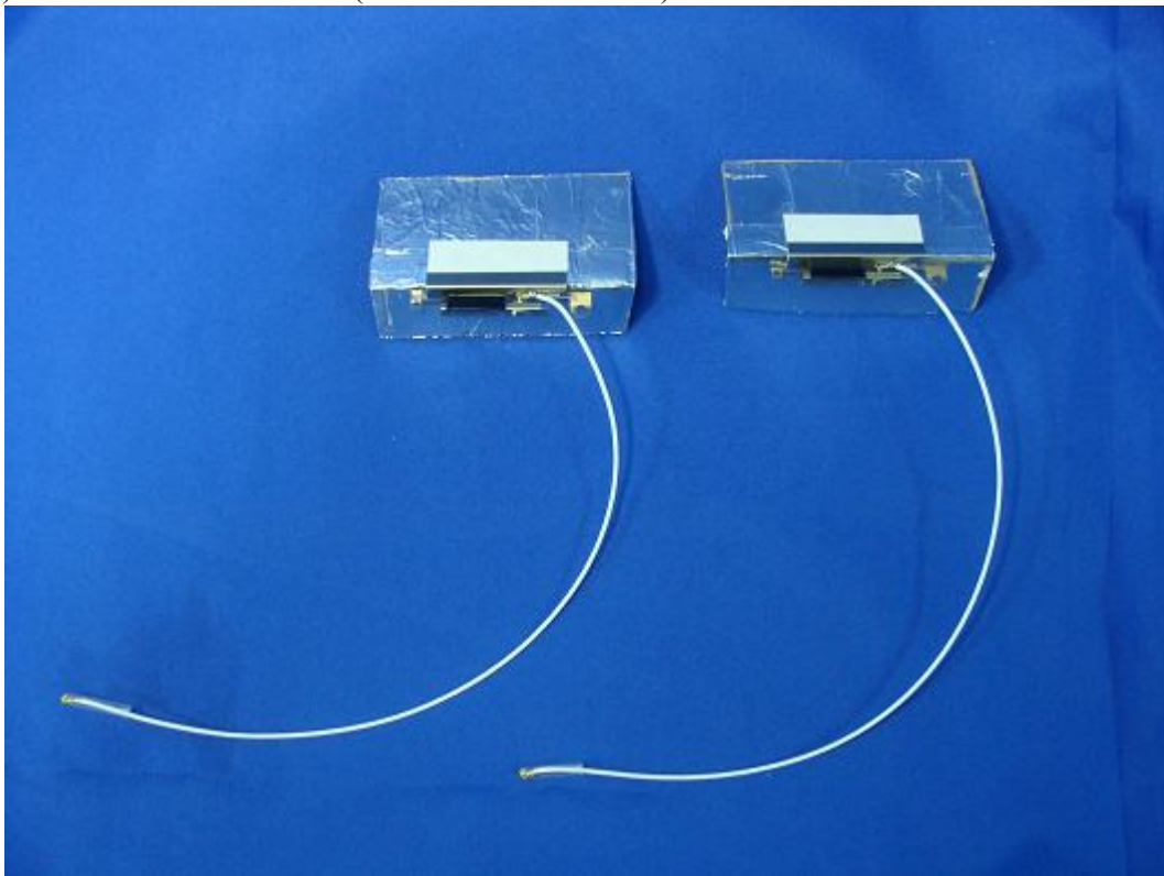
(8) EUT Photo –Antenna 1 (Without metal reflector)
