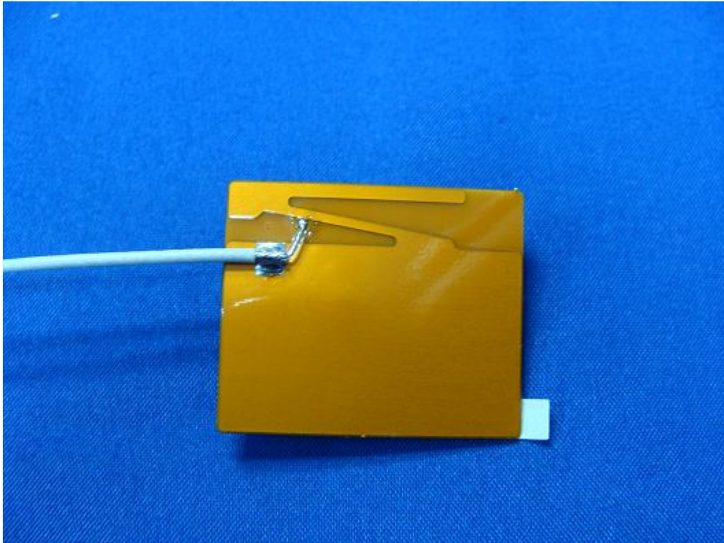
(36) EUT Photo –Antenna 4 (Without metal reflector)
