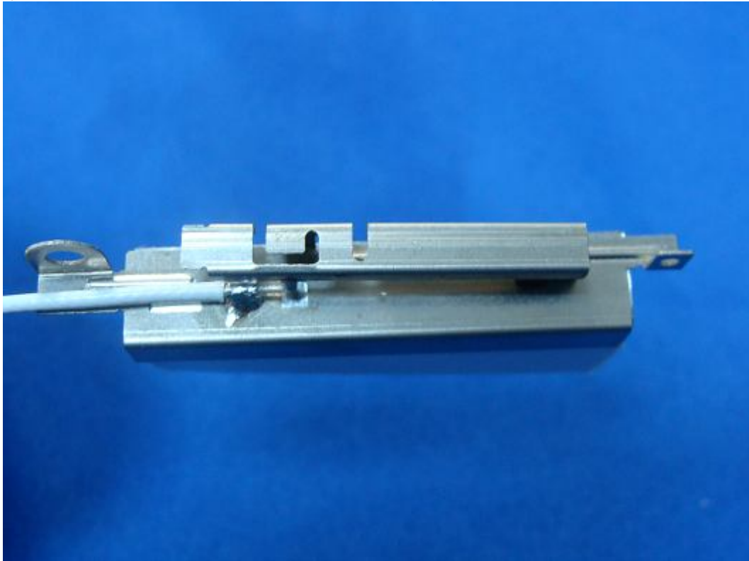
(14) EUT Photo –Antenna 1 (Without metal reflector)
