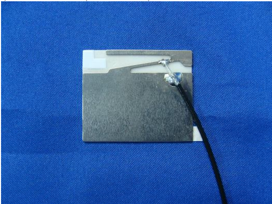
(32) EUT Photo –Antenna 3 (With metal reflector)
