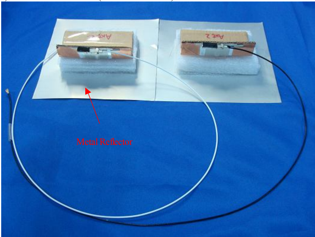
(18) EUT Photo –Antenna 2 (With metal reflector)
