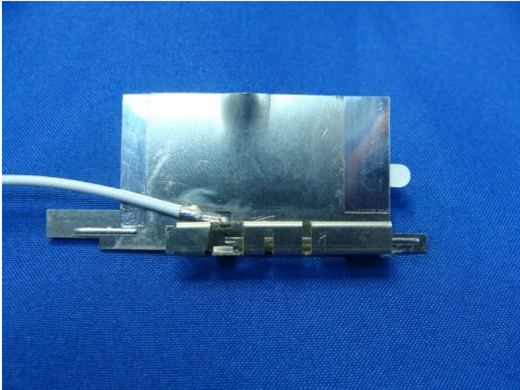
(22) EUT Photo –Antenna 2 (With metal reflector)
