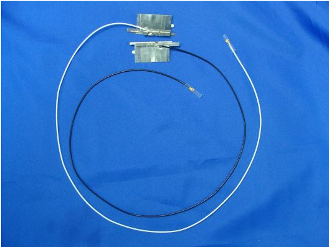
(20) EUT Photo –Antenna 2 (With metal reflector)
