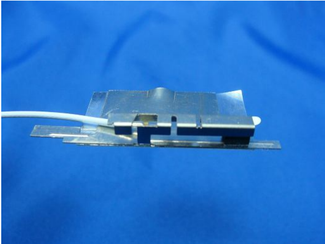
(24) EUT Photo –Antenna 2 (With metal reflector)
