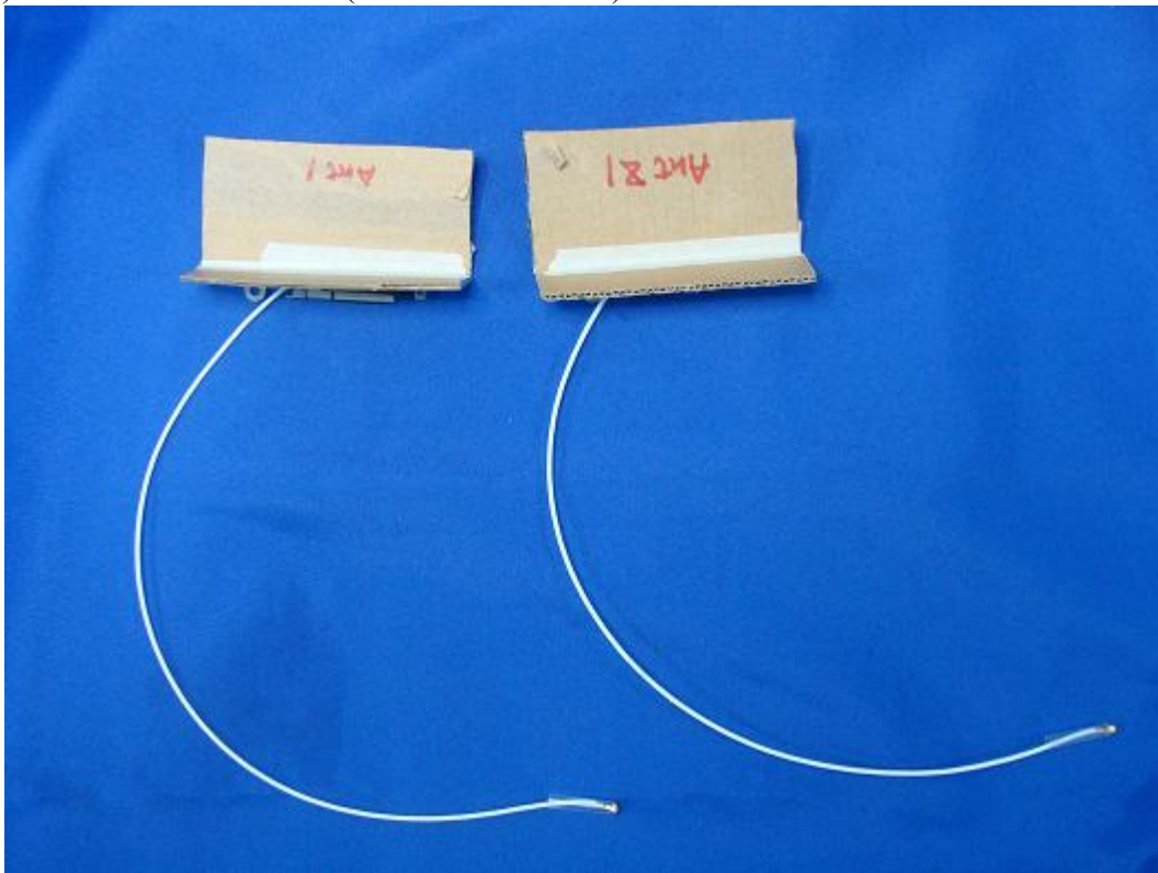
(10) EUT Photo –Antenna 1 (With metal reflector)
