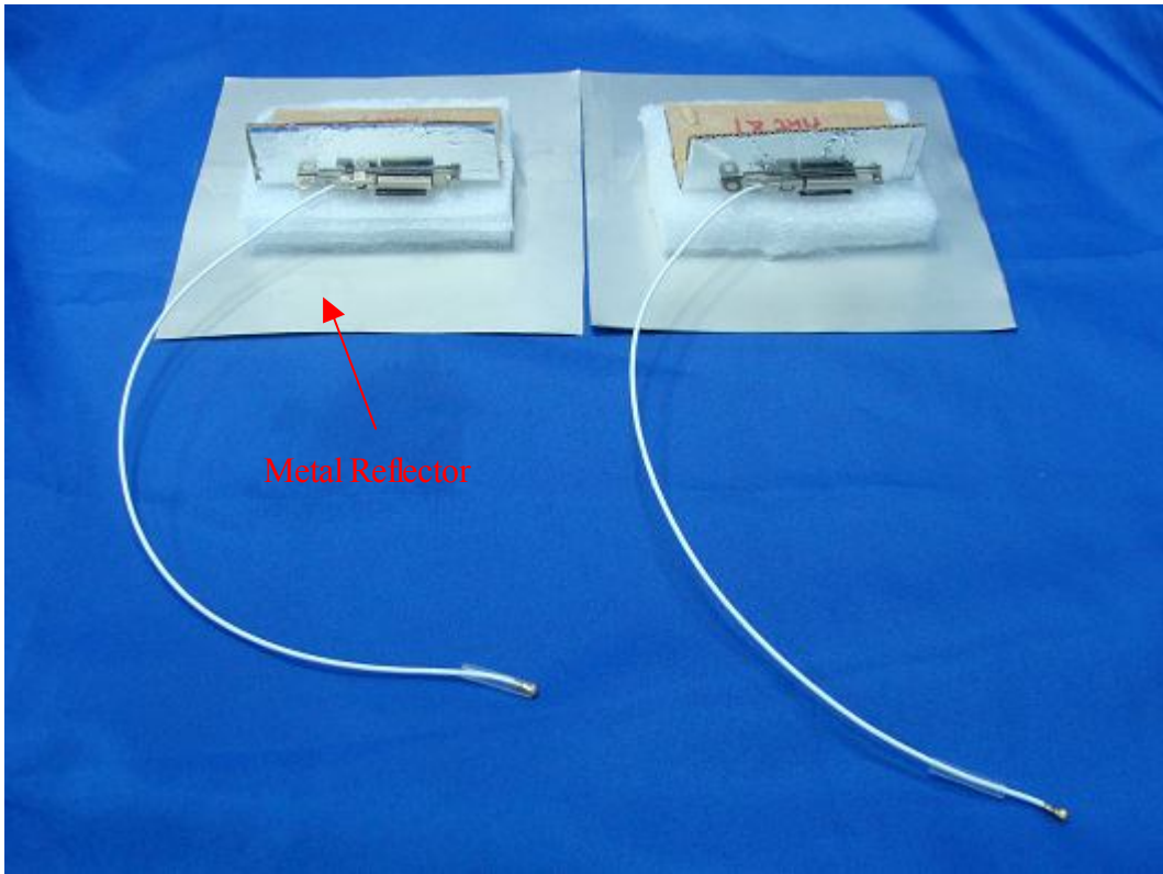
(8) EUT Photo –Antenna 1 (With metal reflector)
