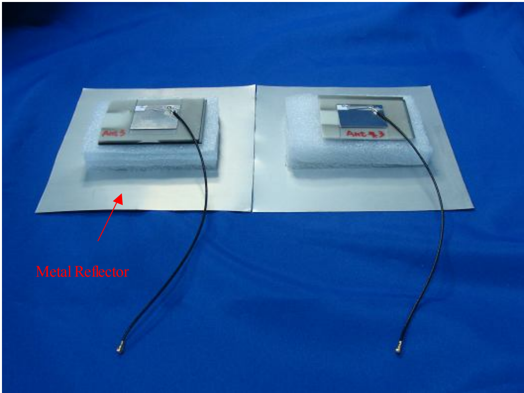
(28) EUT Photo –Antenna 3 (With metal reflector)
