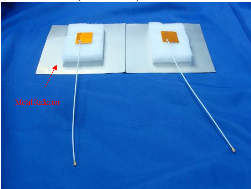
(34) EUT Photo –Antenna 4 (With metal reflector)
