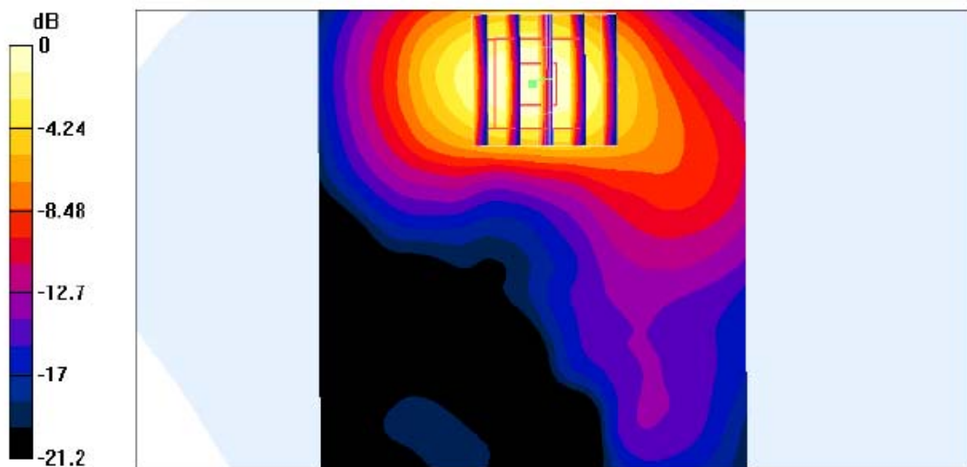
0 dB = 0.127mW/g
