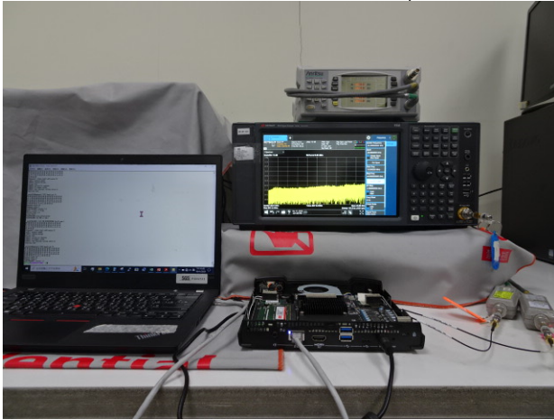
Part 15.407_6E_Radiated_Setup
