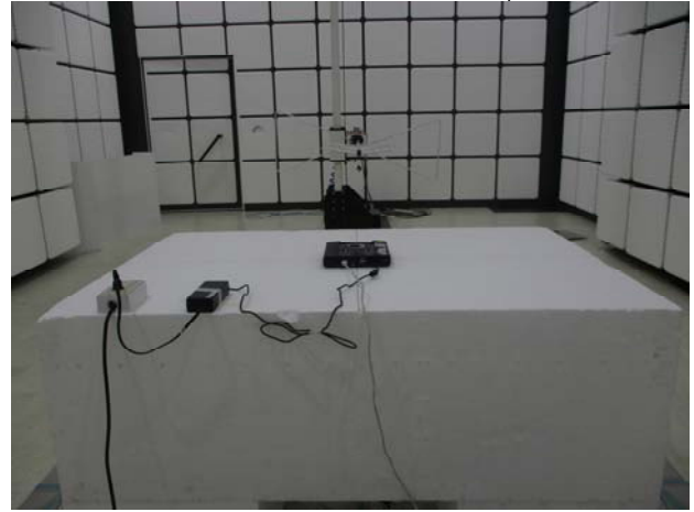
Part 15.247_2.4G_Radiated_Setup
