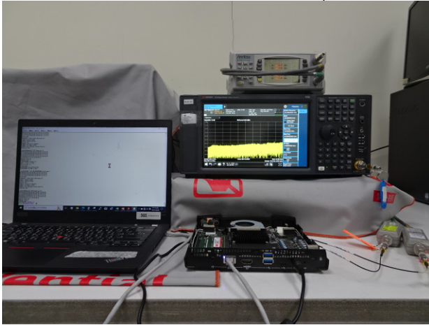
Part 15.247_2.4G_Radiated_Setup
