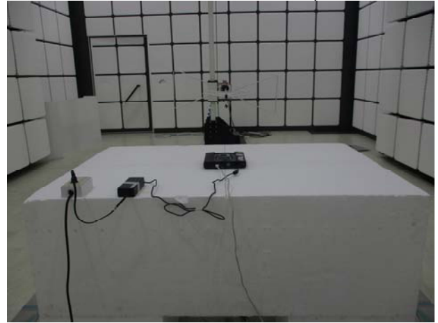
Part 15.247_BT_Radiated_Setup
