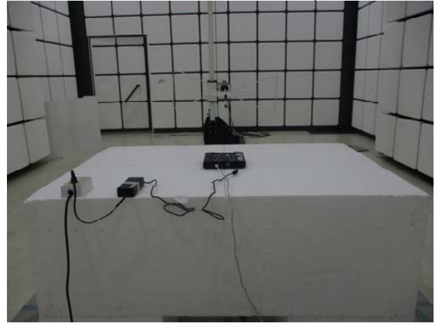
Part 15.407_5G_Radiated_Setup
