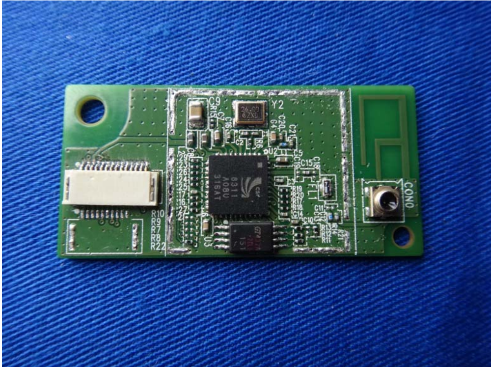
(9) EUT Photo (14 Pin)
