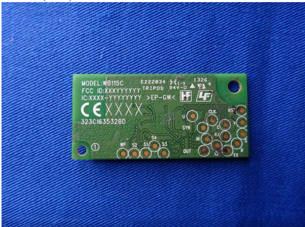
(4) EUT Photo (14 Pin)
