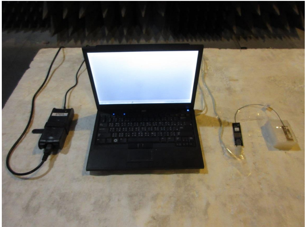
EUT Close-Up
