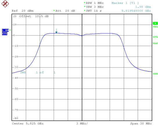
Modulation Type: 802.11a CH165
