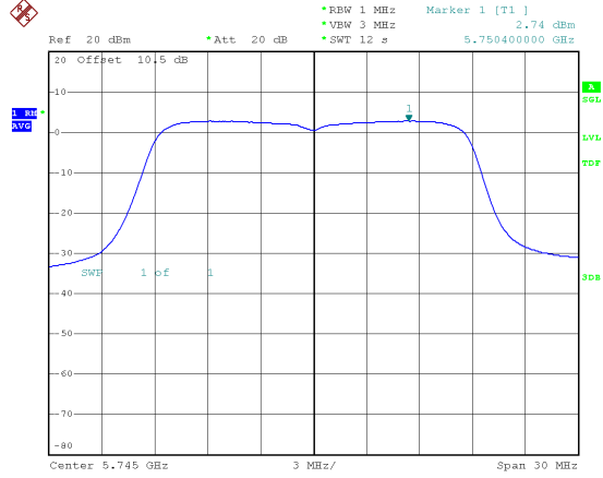
Modulation Type: 802.11ac VHT20 CH149
