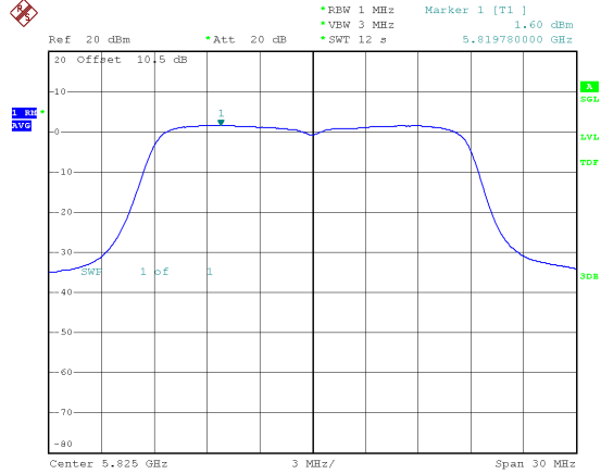
Modulation Type: 802.11ac VHT20 CH165
