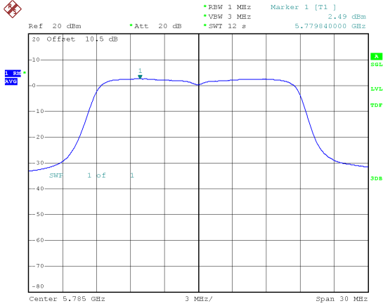
Modulation Type: 802.11ac VHT20 CH157
