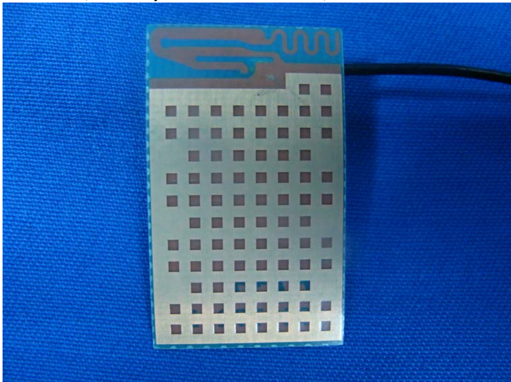
(16) EUT Photo (Antenna: Tyco Electronics / 2174241-2)
