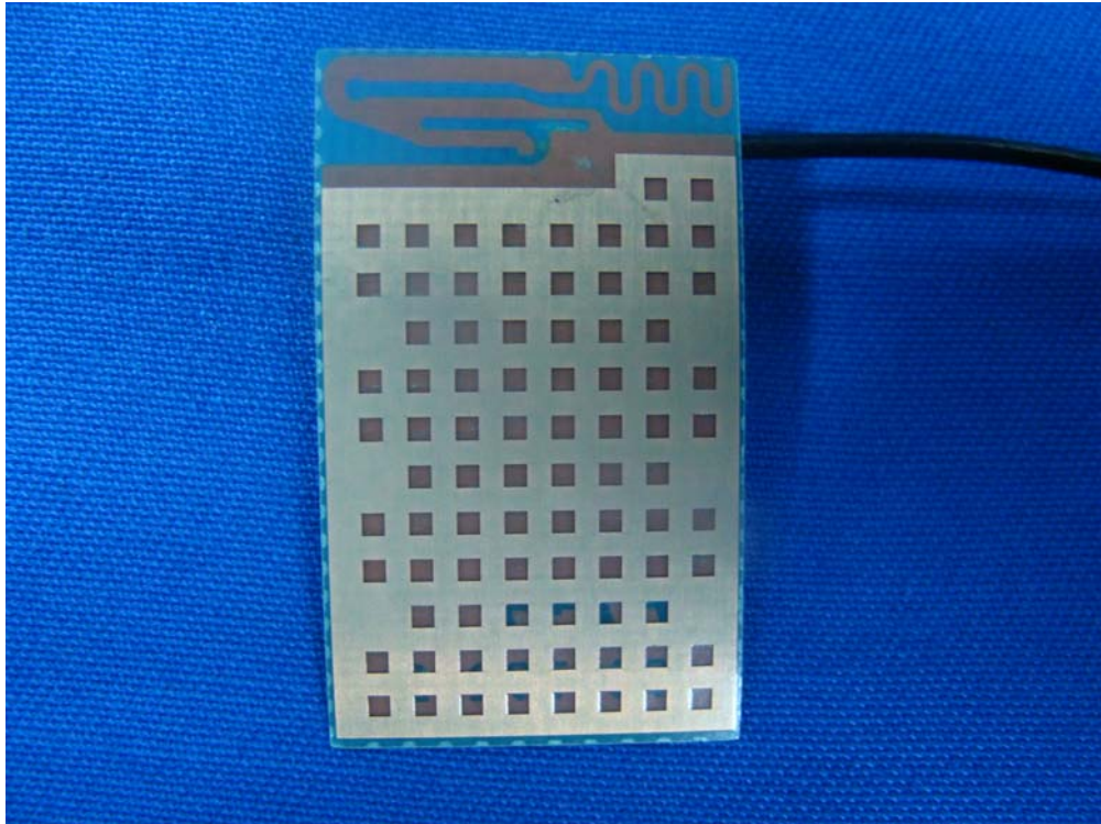
(13) EUT Photo (Antenna: Tyco Electronics / 2174241-1)
