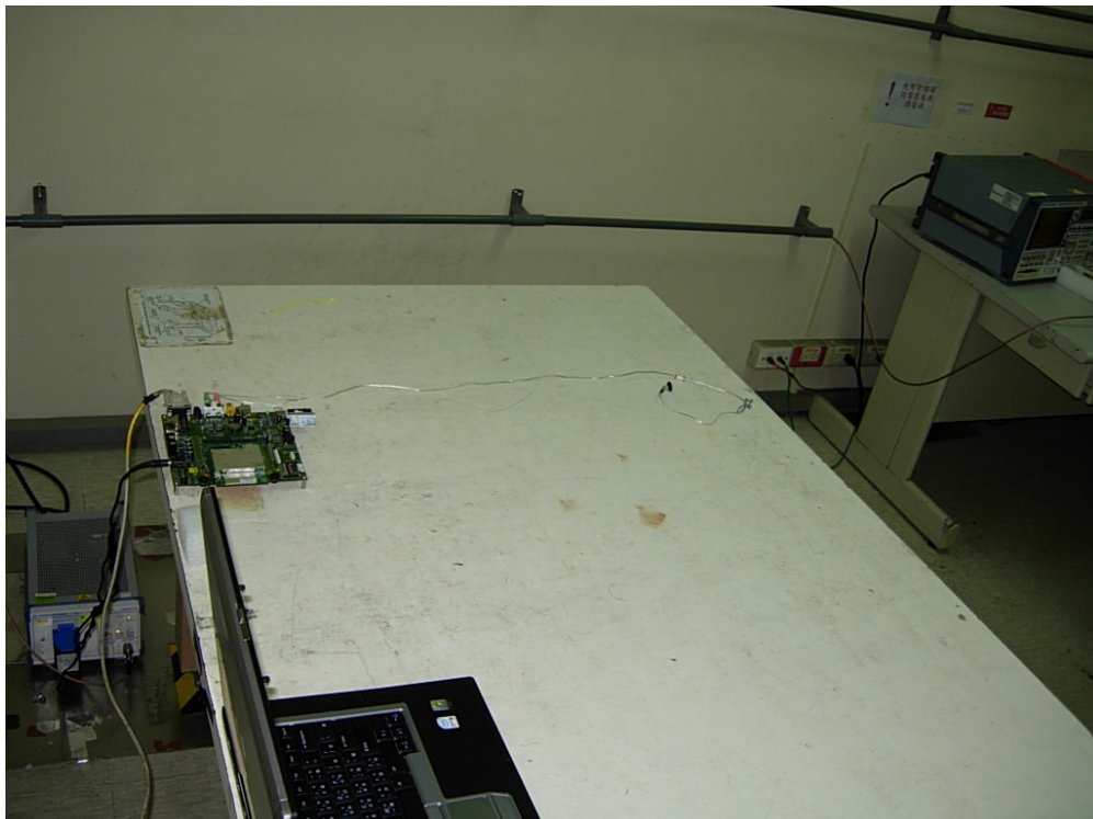
Back View of Conducted Test (Antenna 2)
