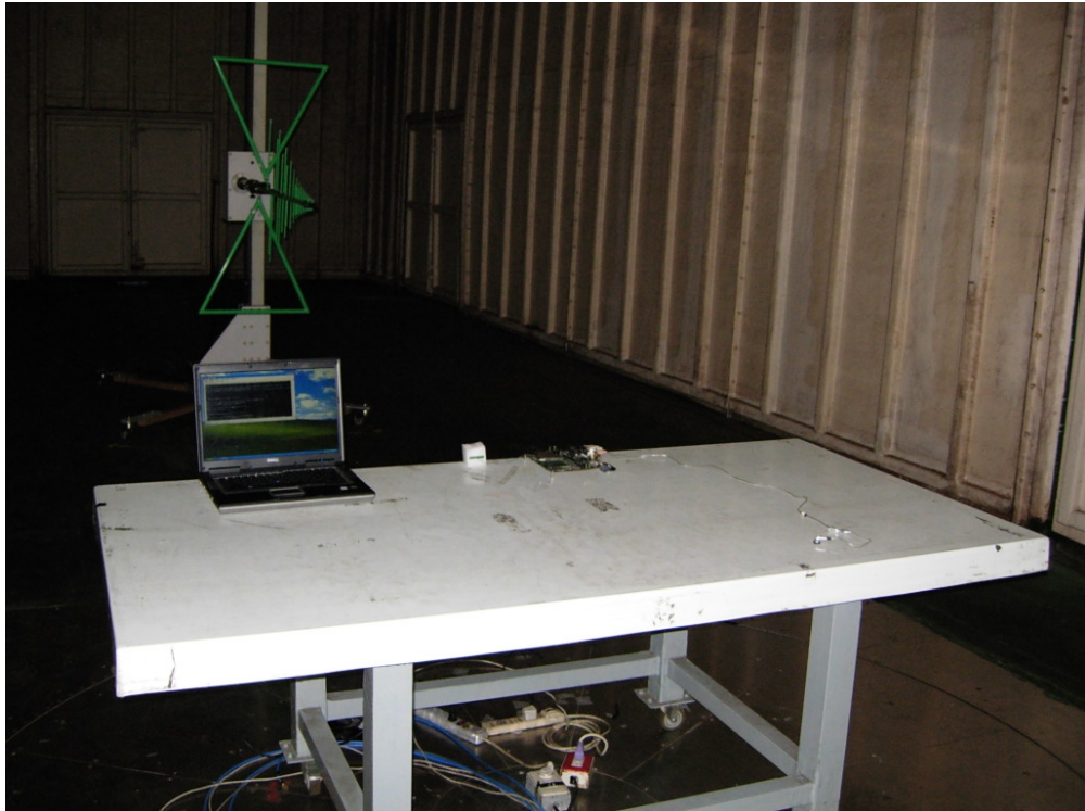
Back View of Radiated Test (Antenna 2)
