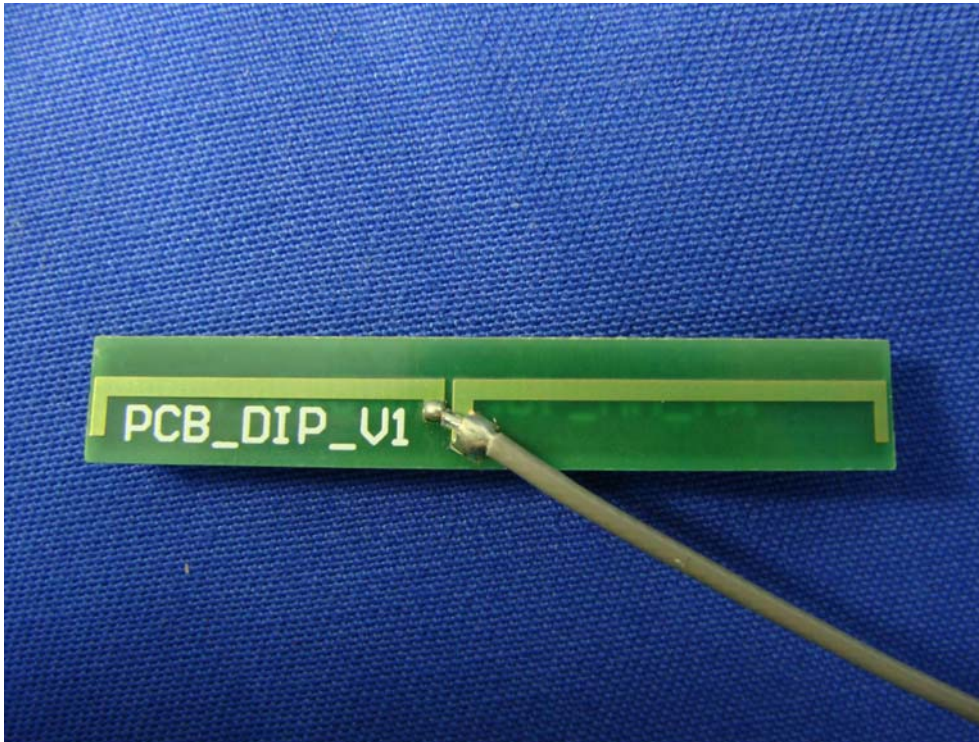
(15) EUT Photo (INPAQ / WA-P-LA-03-034)
