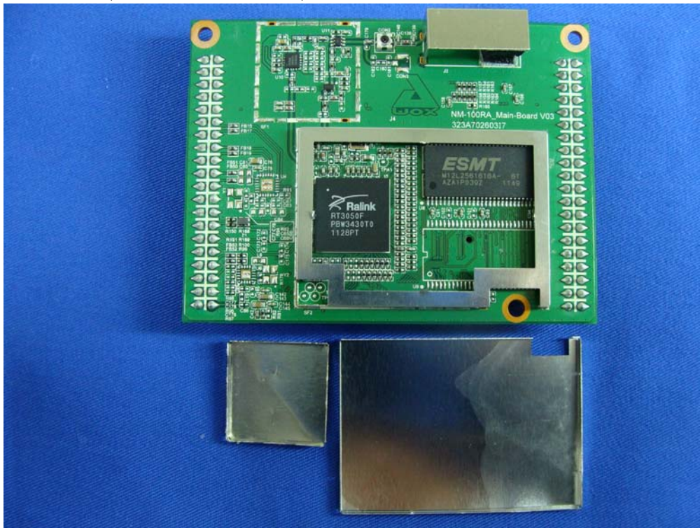
(15) EUT Photo (M/N: AWOXMII0D32)
