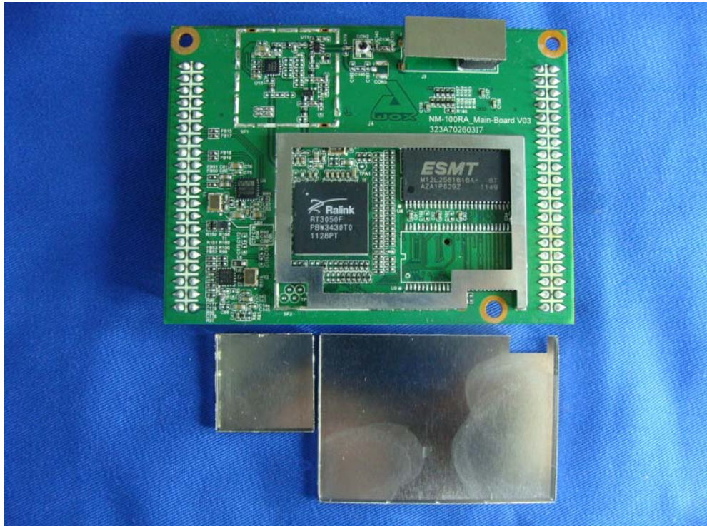
(5) EUT Photo (M/N: AWOXMII0A32)
