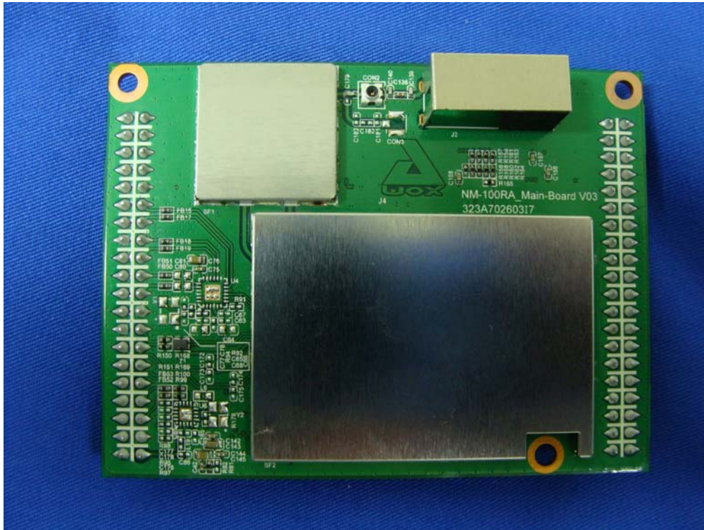
(3) EUT Photo (M/N: AWOXMII0D32)
