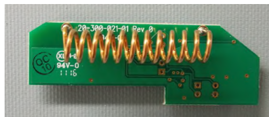
Transmit PCB Rear
