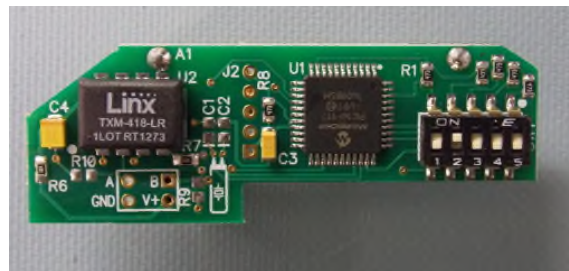
Transmit PCB Rear
